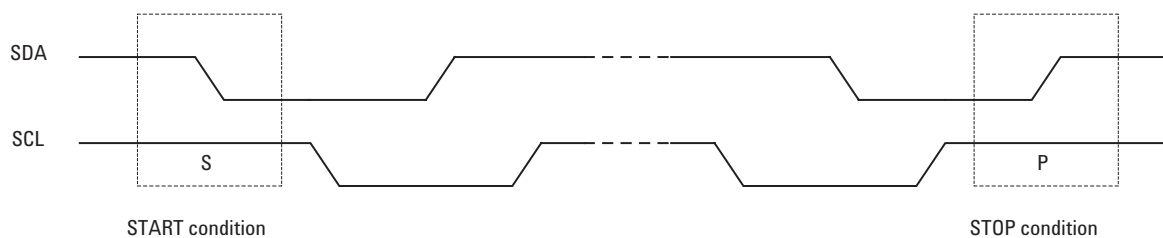
Figure 2. START/STOP Condition
