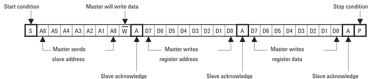
Figure 9. Register Byte Write Protocol
