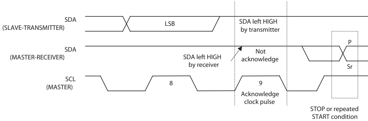
Figure 8. Master-Receiver Acknowledge
