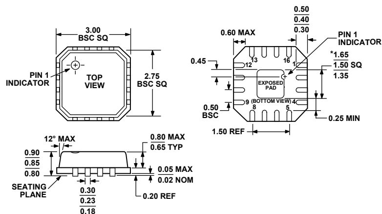
Figure 26. 16-Lead Lead Frame Chip Scale Package [LFCSP_VQ]
