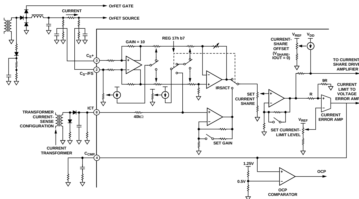
Figure 13. Current Sense
