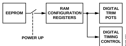
Figure 37. EEPROM Download
