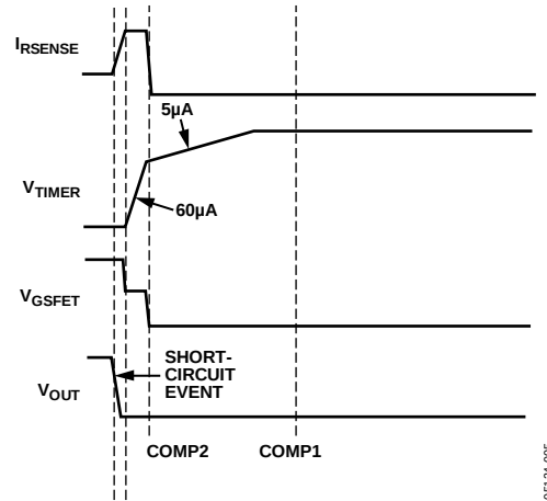
Figure 36. ADM1170-2 Latch Off After Overcurrent Fault
