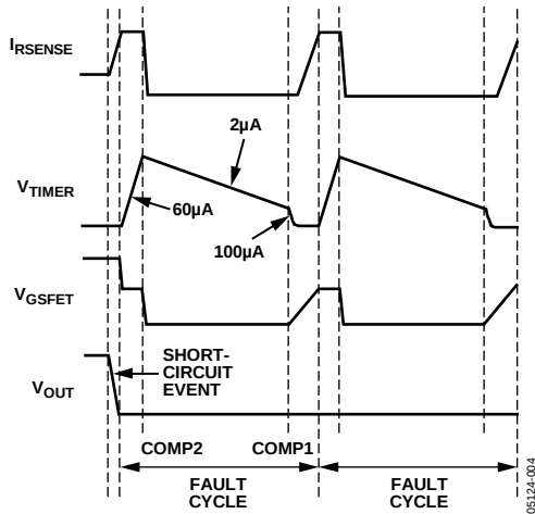
Figure 35. ADM1170-1 Automatic Retry During Overcurrent Fault
