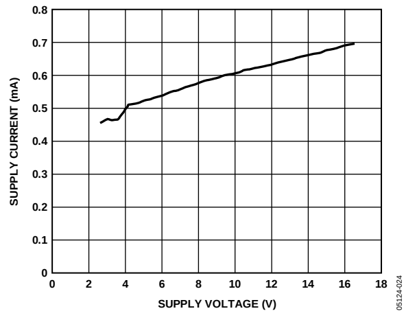
Figure 5. Supply Current vs. Supply Voltage (GATE on)
