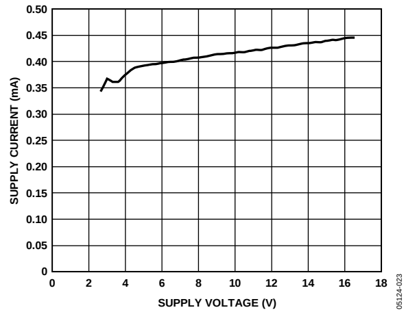
Figure 4. Supply Current vs. Supply Voltage (GATE off)
