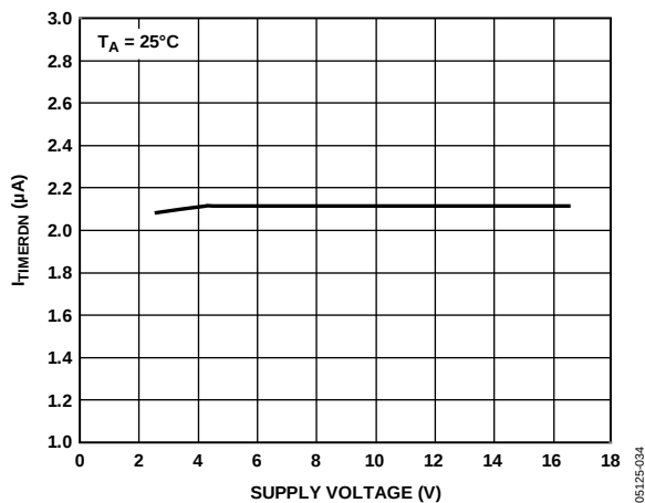
Figure 16. I_{\text{TIMERDN}} (in Cool-Off Cycle) vs. Supply Voltage
