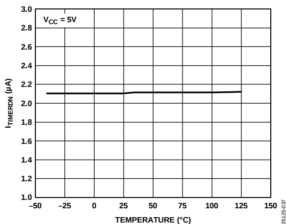
Figure 17. I_{\text{TIMERDN}} (in Cool-Off Cycle) vs. Temperature
