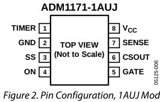
Figure 2. Pin Configuration, 1AUJ Model
