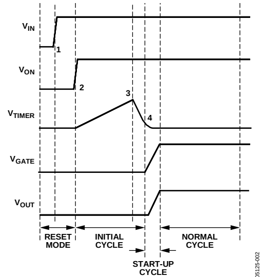
Figure 36. Power-Up Timing
