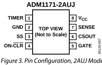
Figure 3. Pin Configuration, 2AUJ Model
