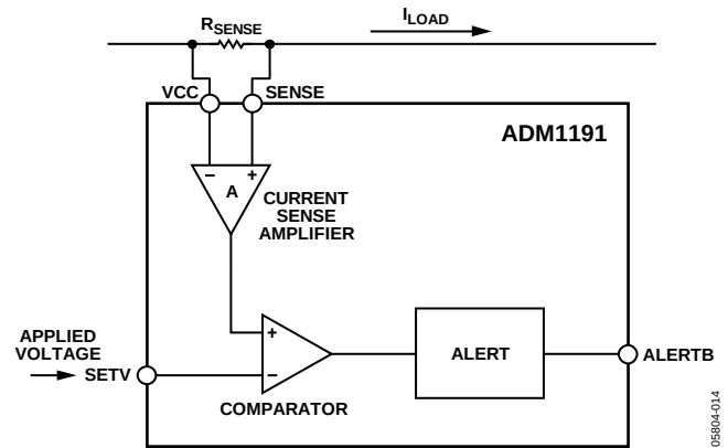
Figure 26. SETV Operation
