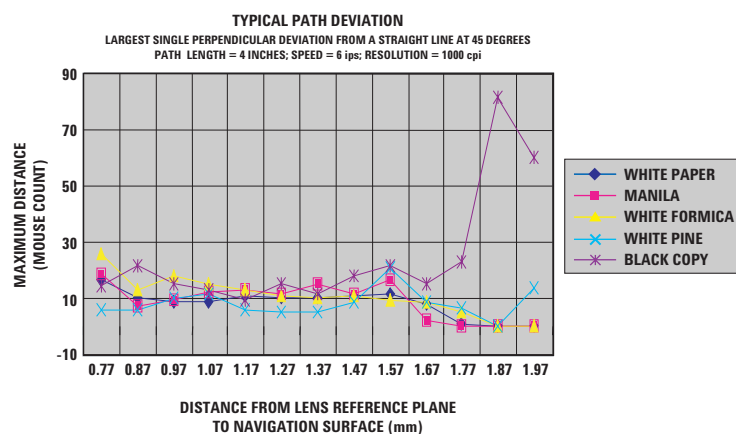
Figure 10. Typical path deviation vs. Z distance (mm)
