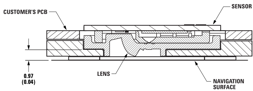
Figure 8b. Distance from lens reference plane to surface (top mount)
