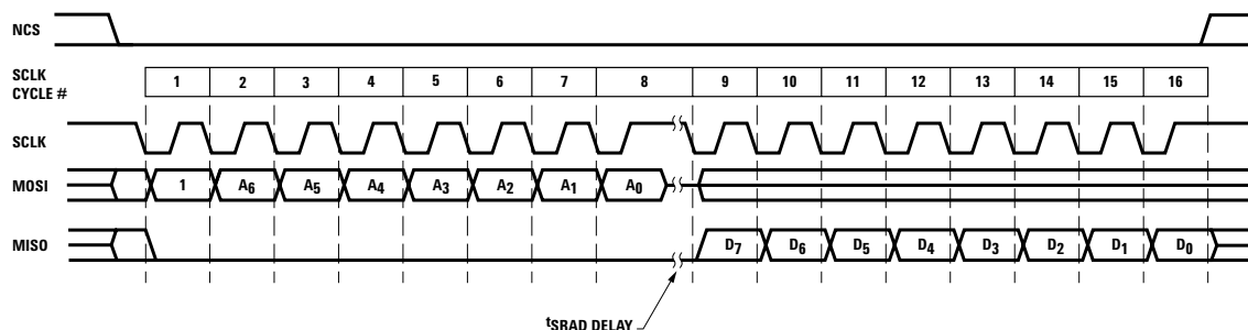
Figure 13. Read operation
