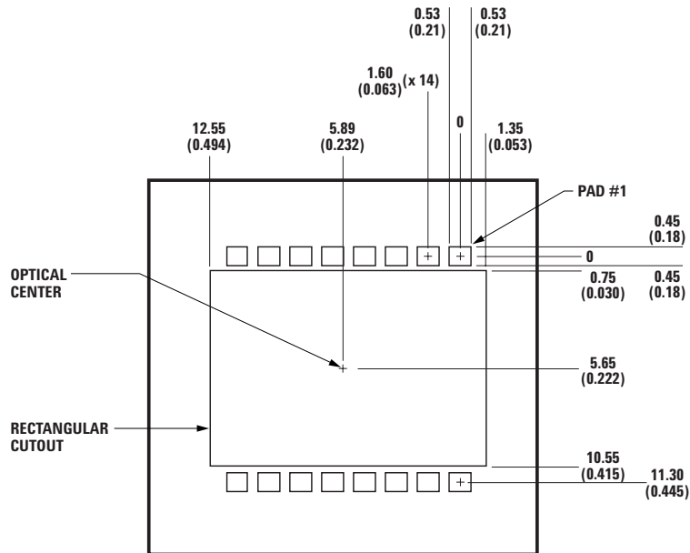
Figure 3. Recommended customer PCB PADOUT and spacing
