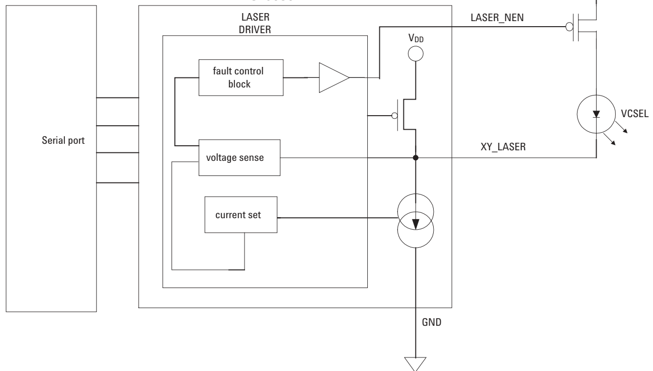
Figure 6. Single Fault Detection and Eye-safety Feature Block Diagram
