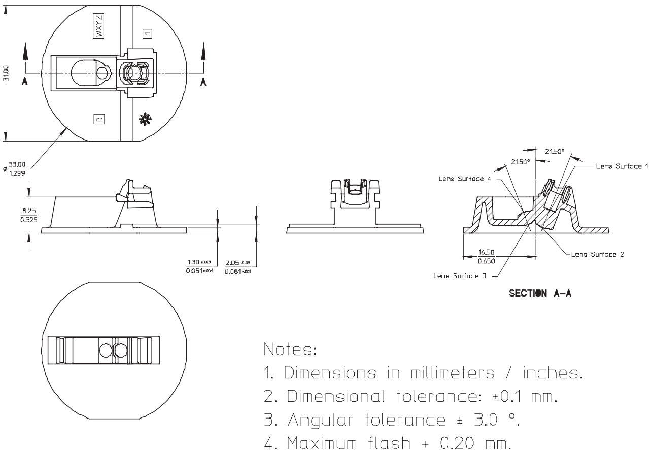
Figure 33. ADNS-6120 laser mouse round lens outline drawings and details
