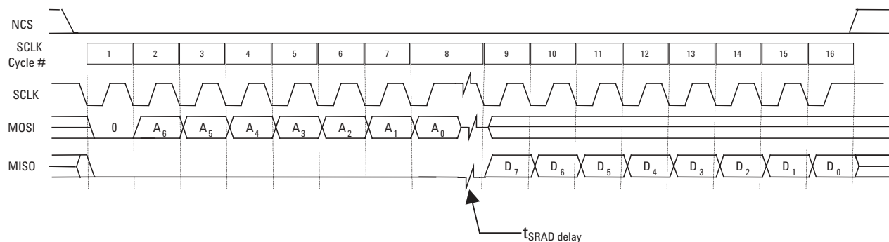
Figure 17. Read Operation
