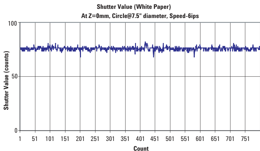
Figure 24. Shutter Values at 800cpi (White Paper)
