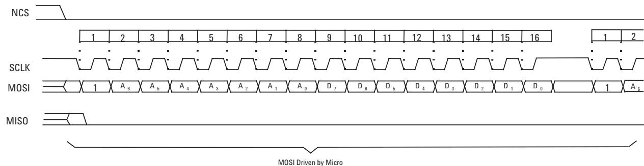
Figure 16. Write Operation
