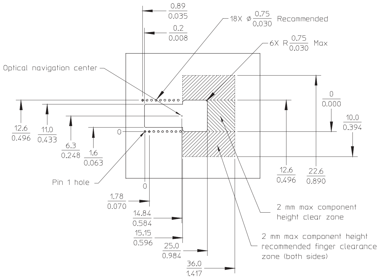
Figure 3. Recommended PCB mechanical cutouts and spacing
