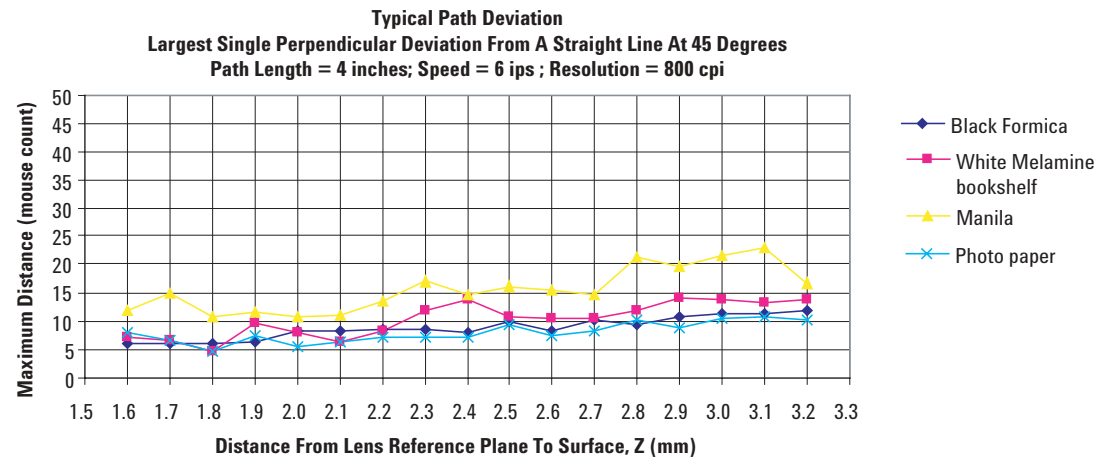
Figure 12. Average Error vs. Distance at 800cpi (mm)
