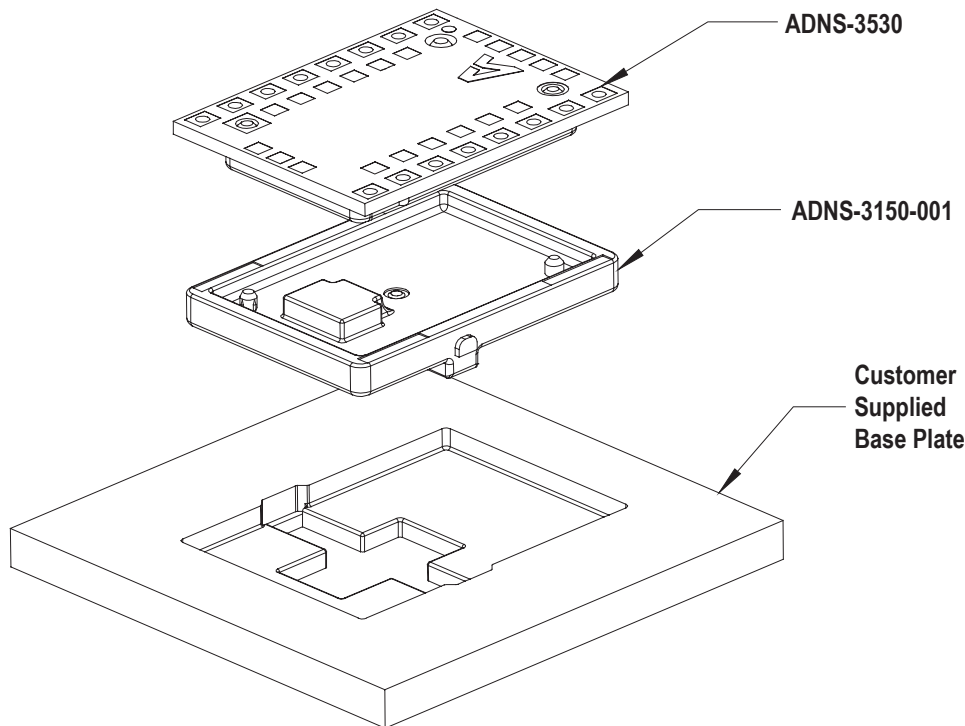
Figure 2. Exploded view drawing of optical tracking engine with ADNB-3532 optical mouse sensor.
