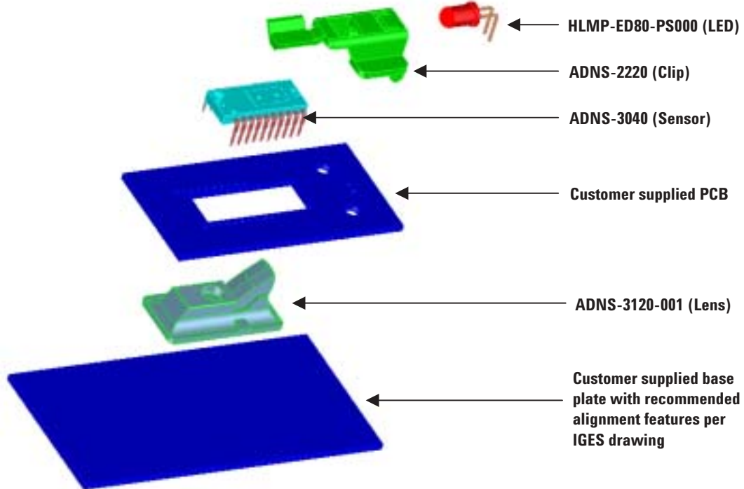
Figure 5. Exploded view
