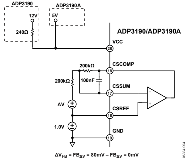
Figure 6. Positioning Voltage
