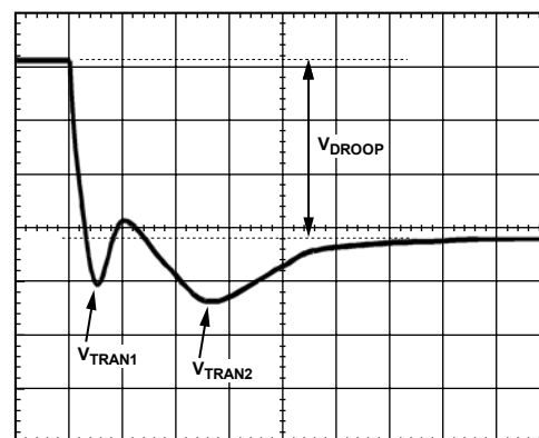
Figure 15. Transient Setting Waveform
