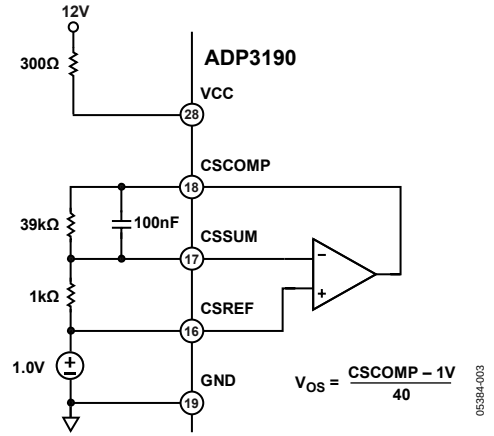
Figure 5. Current Sense Amplifier V_{OS}
