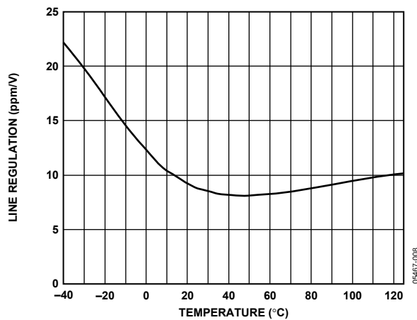
Figure 10. ADR360 Line Regulation vs. Temperature, V_{IN} = 2.45V to 15V
