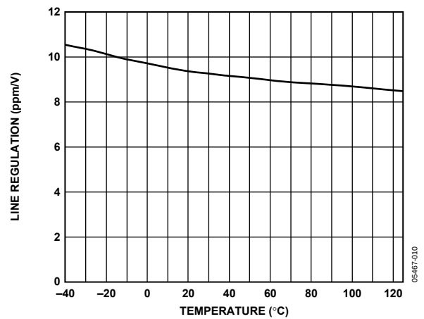
Figure 12. ADR365 Line Regulation vs. Temperature, V_{IN} = 5.3V to 15V
