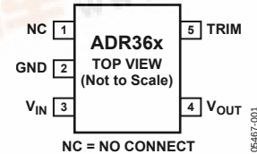
Figure 1. 5-Lead TSOT (UJ Suffix)
