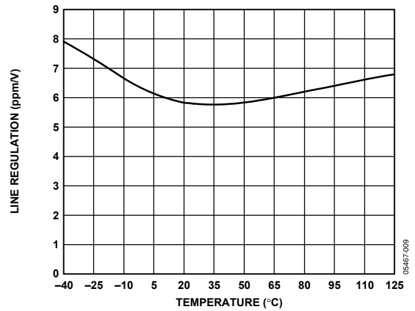
Figure 11. ADR361 Line Regulation vs. Temperature, V_{IN} = 2.8V to 15V
