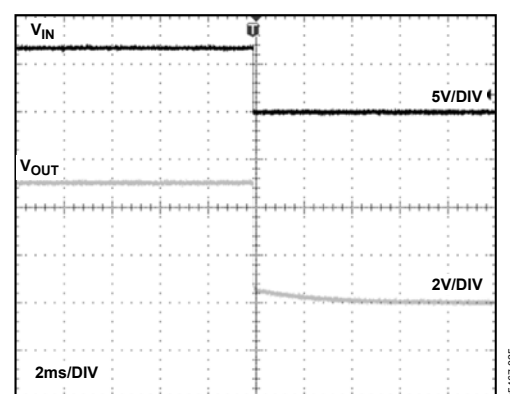
Figure 31. ADR361 Turn-Off Response, 0.1 \mu F Output Capacitor
