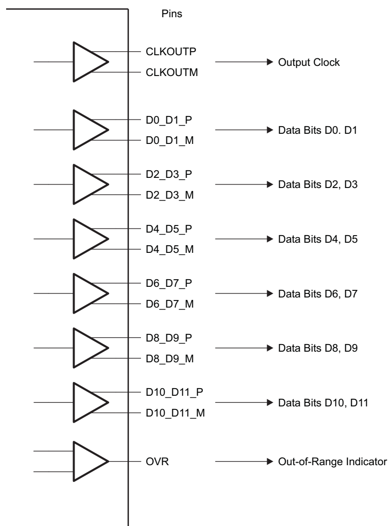
Figure 45. DDR LVDS Outputs
