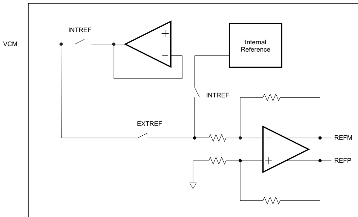
Figure 41. Reference Section
