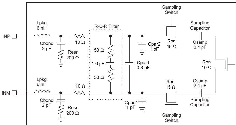
Figure 37. Input Stage
