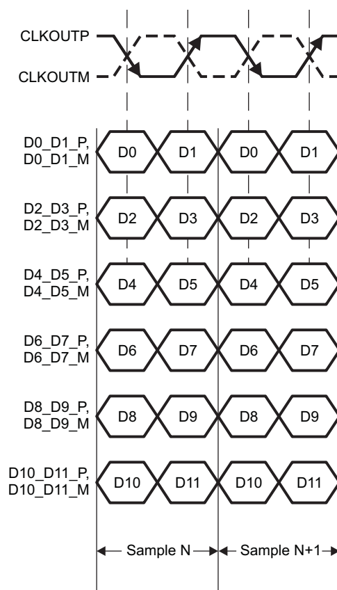
Figure 46. DDR LVDS Interface
