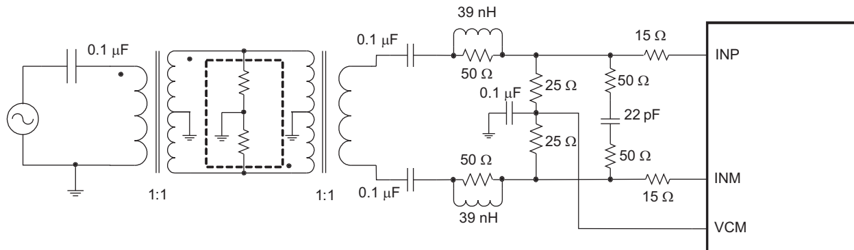
Figure 99. Drive Circuit with Low Bandwidth (for low input frequencies)
