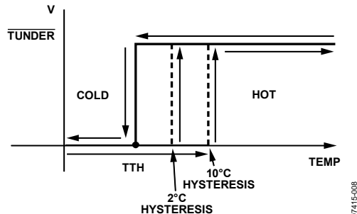
Figure 20. ADT6401 \overline{TUNDER} Transfer Function
