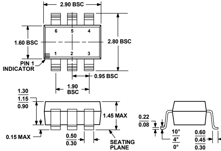
Figure 23. 6-Lead Small Outline Transistor Package [SOT-23] (RJ-6)
