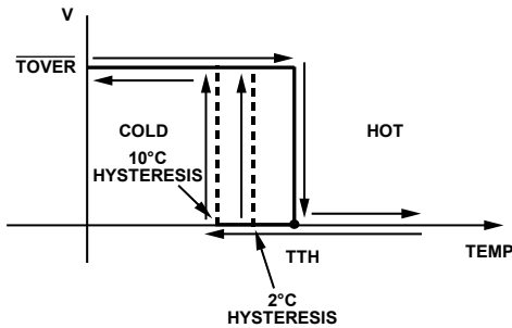
Figure 18. ADT6401 \overline{TOVER} Transfer Function
