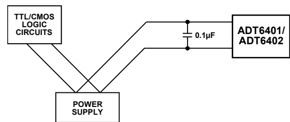
Figure 22. Separate Traces Used to Reduce Power Supply Noise
