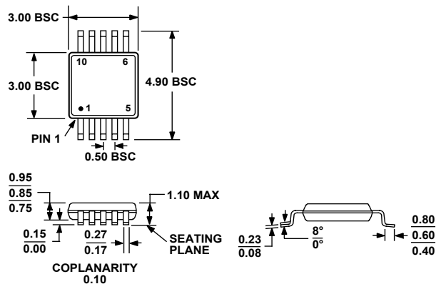
Figure 26. 10-Lead Mini Small Outline Package (MSOP)
