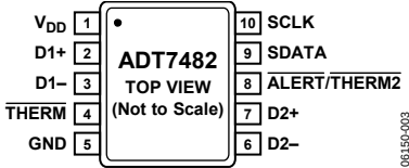
Figure 3. Pin Configuration
