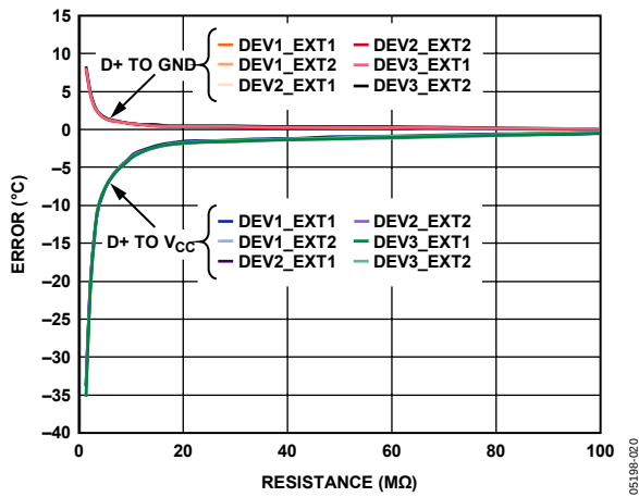
Figure 10. Remote Temperature Error vs. PCB Resistance
