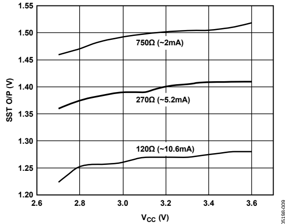
Figure 4. SST O/P Level vs. Supply Voltage
