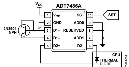
Figure 20. ADT7486A Typical Application Schematic
