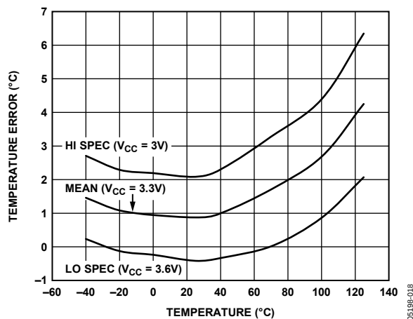
Figure 6. Local Temperature Error
