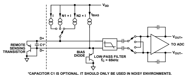
Figure 16. Signal Conditioning for Remote Diode Temperature Sensors
