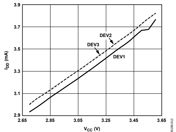
Figure 8. Supply Current vs. Voltage
