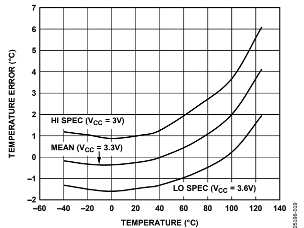
Figure 9. Remote Temperature Error
