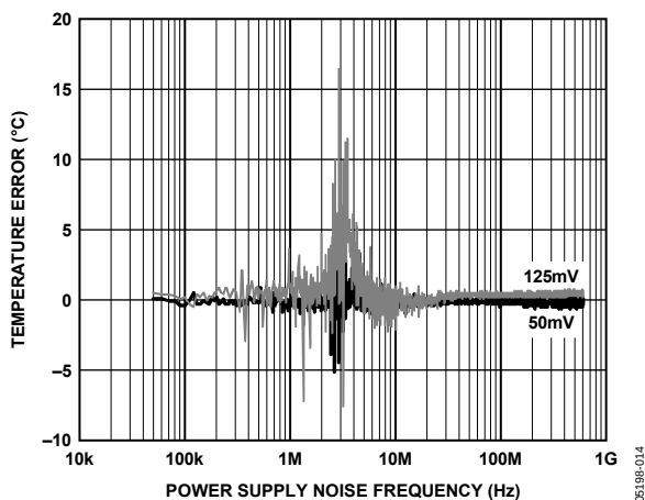
Figure 12. Local Temperature Error vs. Power Supply Noise
