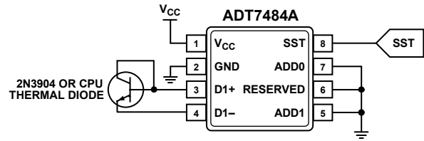
Figure 19. ADT7484A Typical Application Schematic
