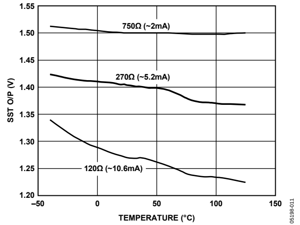
Figure 7. SST O/P Level vs. Temperature
