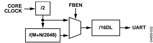
Figure 61. Baud Rate Generation Options
