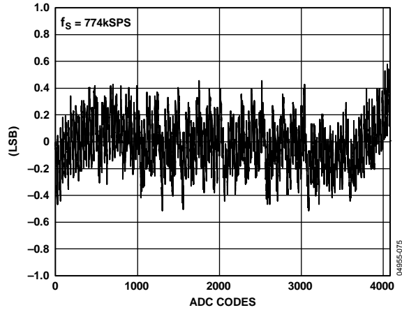
Figure 16. Typical INL Error, f_S = 774 kSPS
