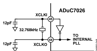
Figure 77. External Parallel Resonant Crystal Connections
