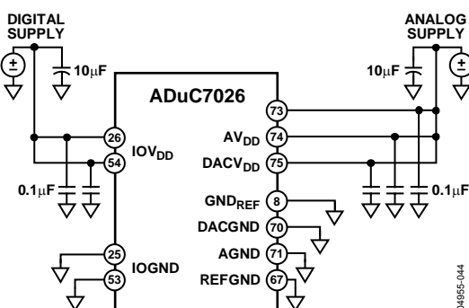
Figure 73. External Dual Supply Connections
