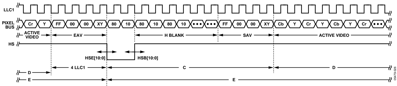
Figure 26. HS Timing
