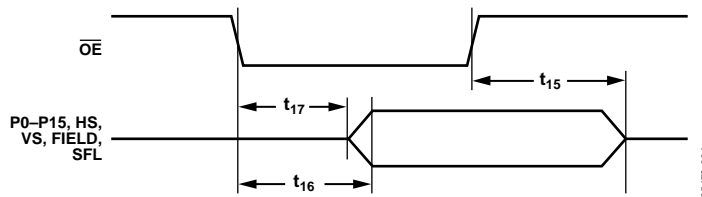
Figure 4. \overline{\text{OE}} Timing
