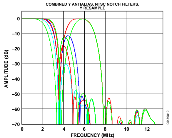
Figure 19. NTSC Notch Filter Responses
