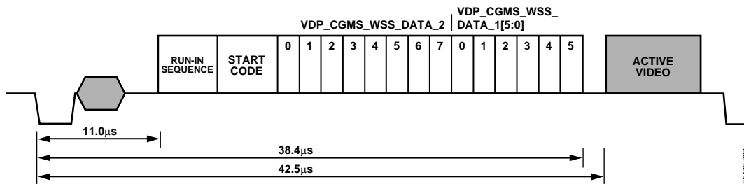
Figure 37. WSS Waveform
