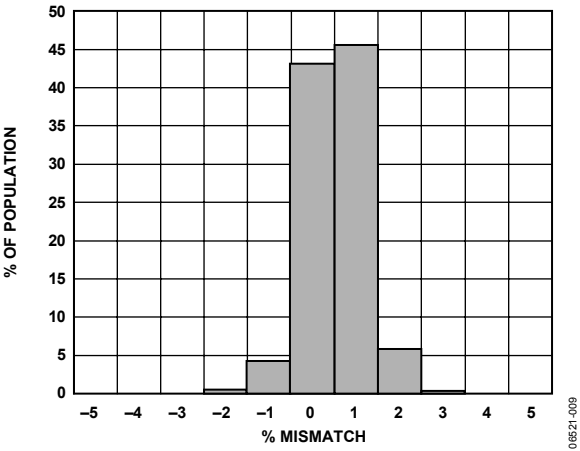
Figure 10. Self-Test Mismatch at 25°C ( V_{RATIO} = 5\text{ V} )
