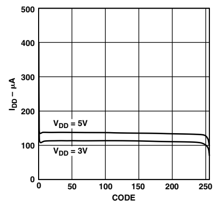
Figure 10. Supply Current vs. Code
