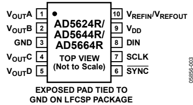
Figure 3. Pin Configuration
