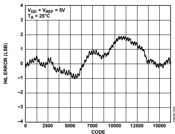
Figure 5. INL AD5644R, External Reference
