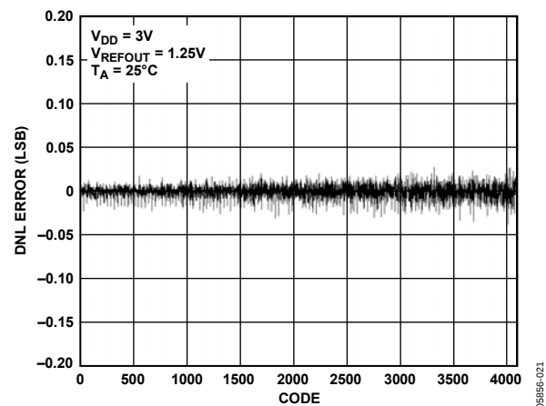
Figure 21. DNL AD5624R-3, Internal Reference
