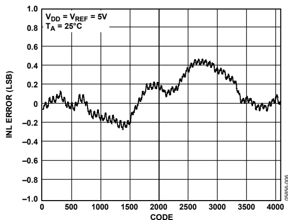
Figure 6. INL AD5624R, External Reference
