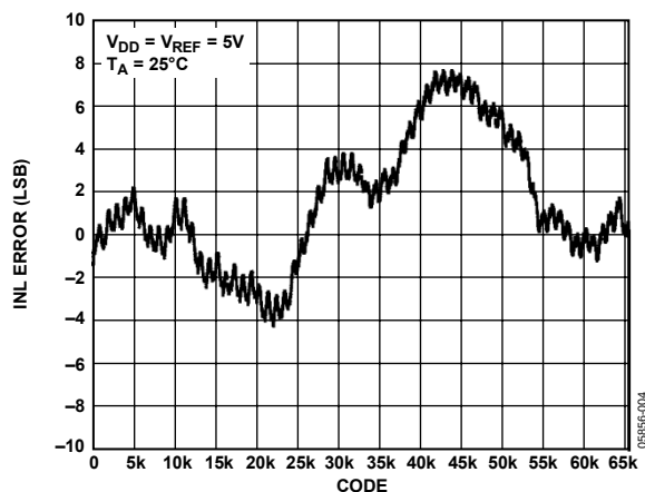
Figure 4. INL AD5664R, External Reference
