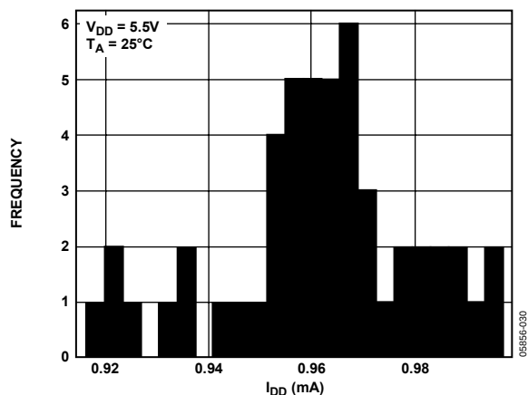
Figure 30. I_{DD} Histogram with Internal Reference, V_{REFOUT} = 2.5 V
