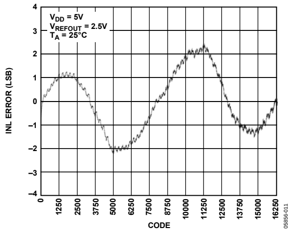
Figure 11. INL AD5644R-5, Internal Reference
