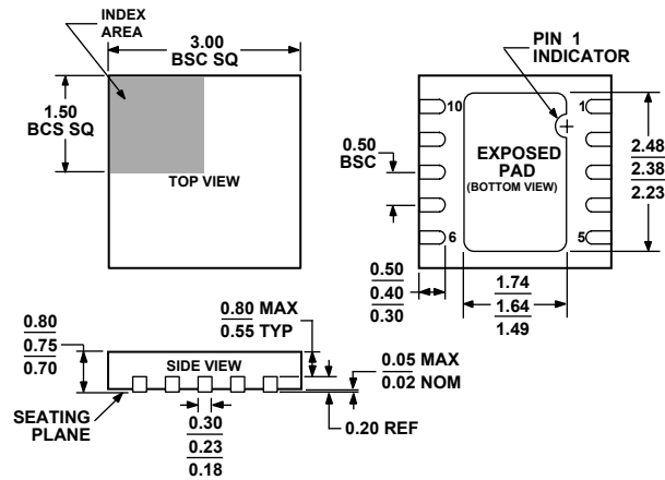
Figure 64. 10-Lead Lead Frame Chip Scale Package [LFCSP_WD] 3 mm × 3 mm Body, Very Very Thin, Dual Lead (CP-10-9) Dimensions shown in millimeters
