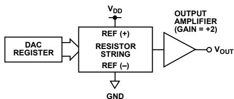
Figure 50. DAC Architecture
