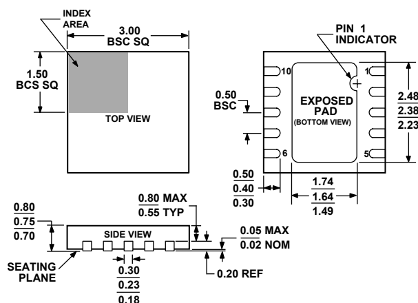
Figure 69. 10-Lead Lead Frame Chip Scale Package [LFCSP_WD] 3 mm x 3 mm Body, Very Very Thin, Dual Lead (CP-10-9)
