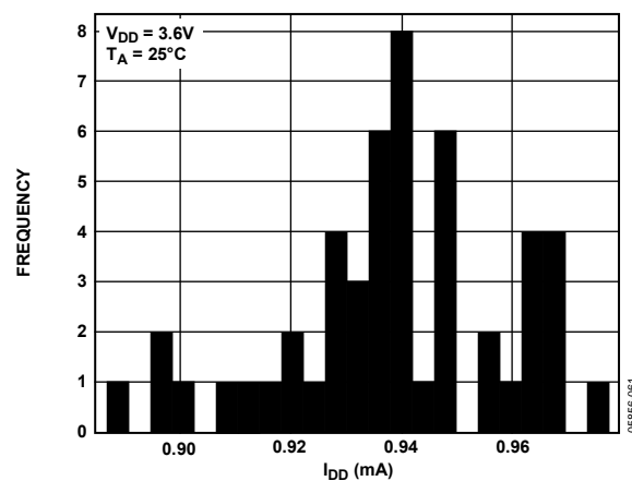
Figure 32. I_{DD} Histogram with Internal Reference, V_{REFOUT} = 1.25\text{ V}
