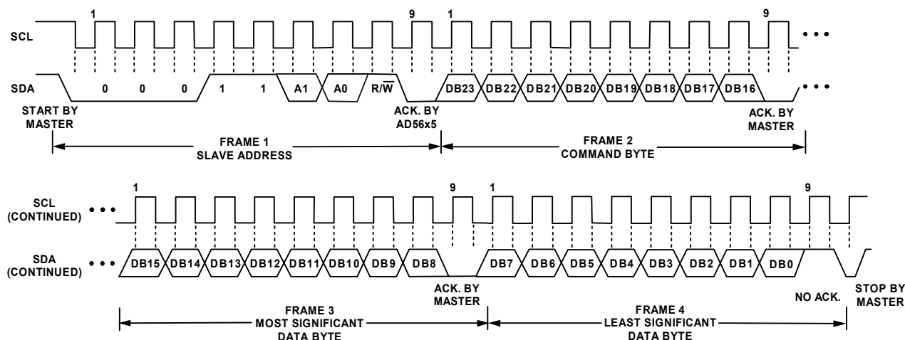
Figure 54. I²C Read Operation(10-Pin Package)
