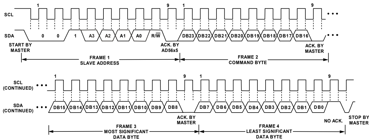
Figure 55. I²C Read Operation(14-Pin Package)
