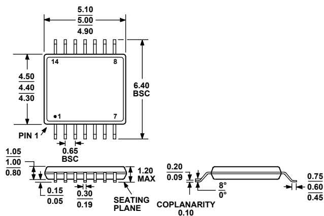
Figure 70. 14-Lead Thin Shrink Small Outline Package [TSSOP] (RU-14)
