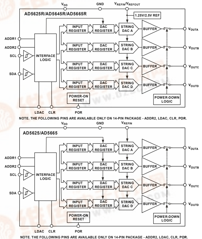
Figure 1. Functional Block Diagrams
