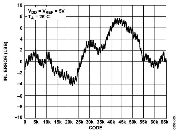
Figure 4. INL AD5665, External Reference
