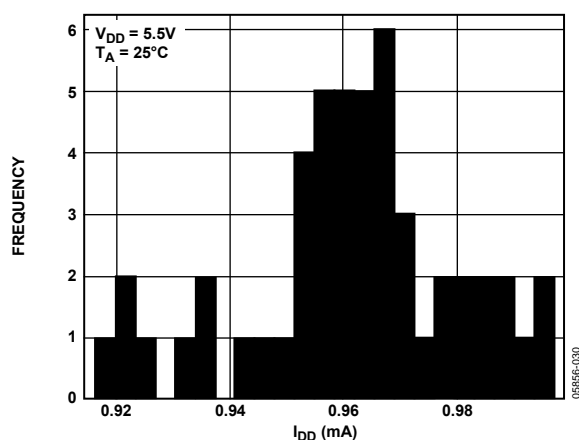
Figure 30. I_{DD} Histogram with Internal Reference, V_{REFOUT} = 2.5\text{ V}
