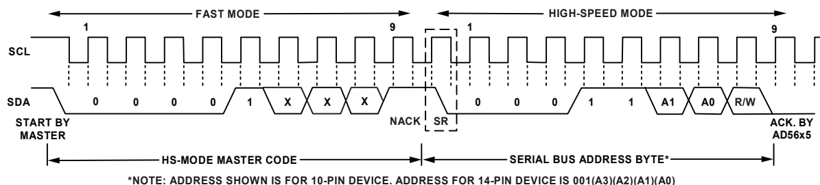
Figure 56. Placing the AD56x5 in High-Speed Mode
