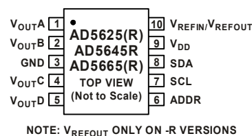
Pin Configuration (10-pin)
