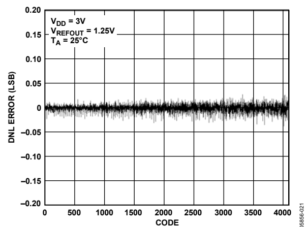
Figure 21. DNL AD5625R, 1.25V Internal Reference
