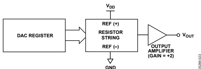
Figure 40. DAC Architecture
