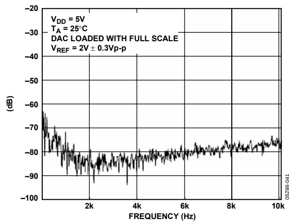
Figure 36. Total Harmonic Distortion
