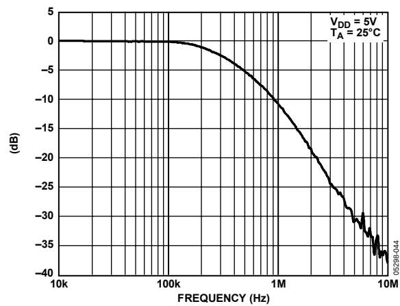
Figure 39. Multiplying Bandwidth
