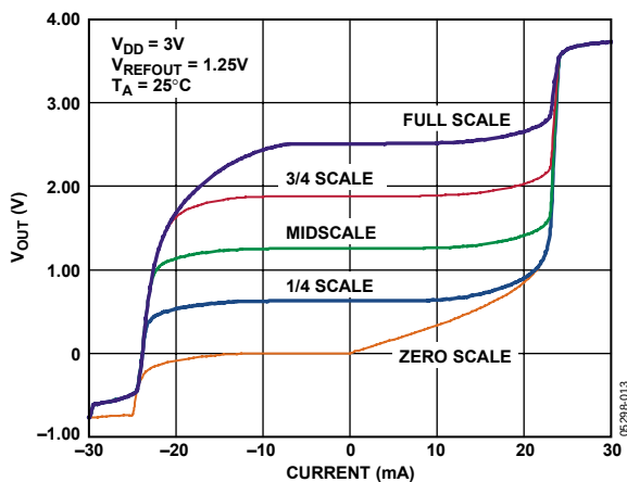
Figure 20. Source and Sink Current Capability with V_{DD} = 5\text{ V}
