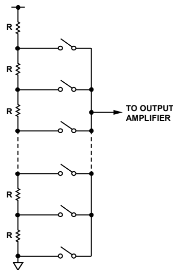
Figure 41. Resistor String
