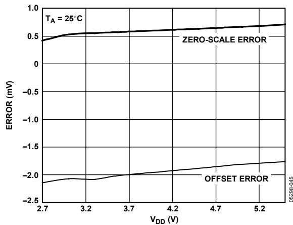
Figure 15. Zero-Scale Error and Offset Error vs. Supply Voltage
