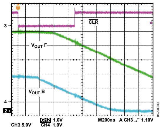
Figure 38. Hardware \overline{CLR}
