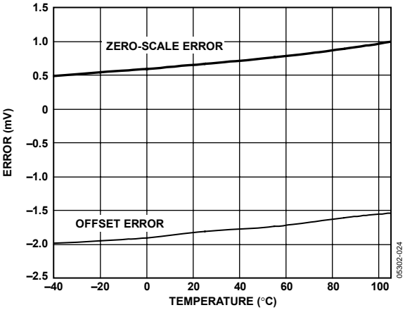
Figure 8. Zero-Scale Error and Offset Error vs. Temperature
