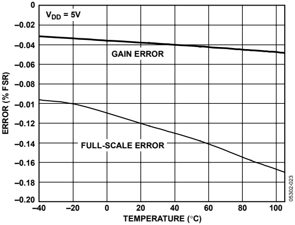
Figure 7. Gain Error and Full-Scale Error vs. Temperature
