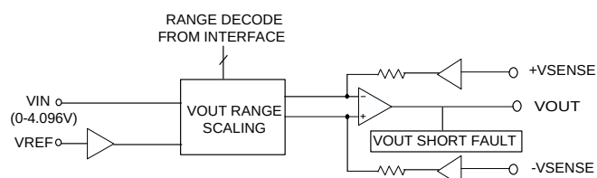
Figure 12. Voltage Output
