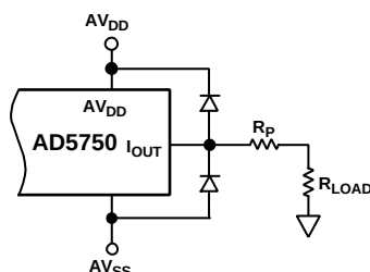
Figure 15. Output Transient Voltage Protection
