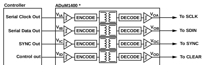
Figure 16. Isolated Interface
