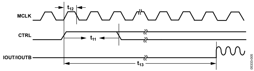
Figure 5. CTRL Timing
