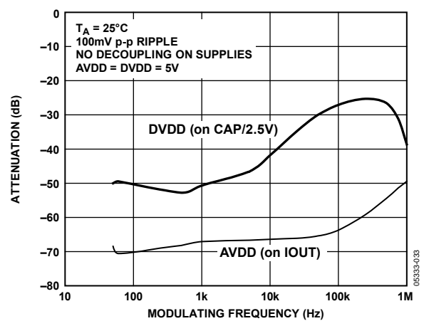
Figure 20. PSSR
