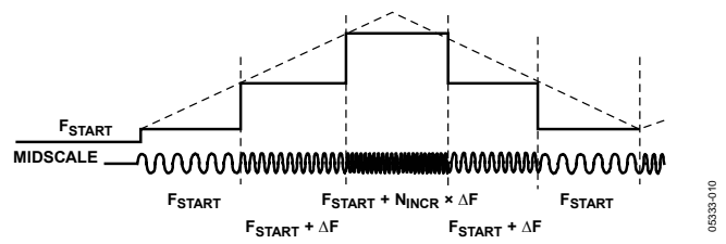
Figure 32. Triangular-Sweep Profile
