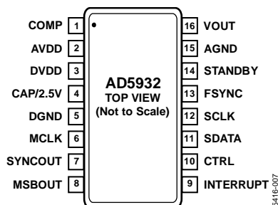
Figure 7. Pin Configuration
