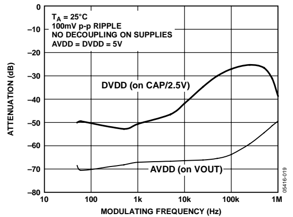
Figure 19. PSSR
