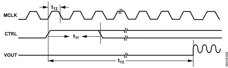
Figure 5. CTRL Timing
