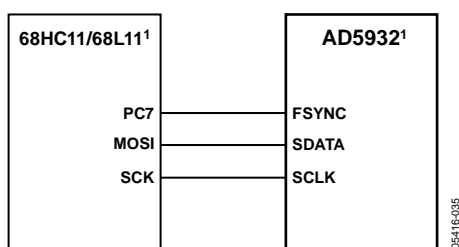
Figure 35. 68HC11/68L11 to AD5932 Interface
