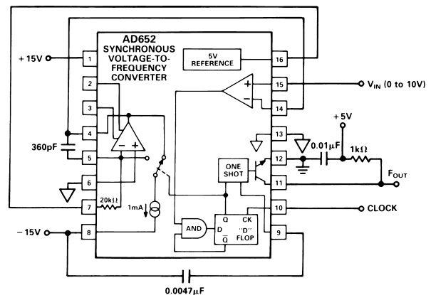
Figure 29. Delta Modulator
