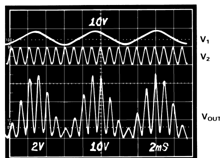
Figure 19. Multiplier Waveforms
