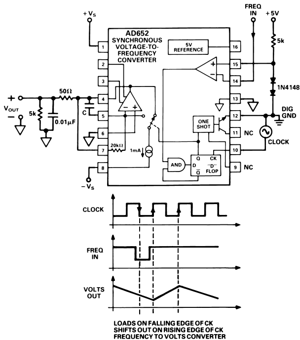
Figure 17. Frequency-to-Voltage Converter
