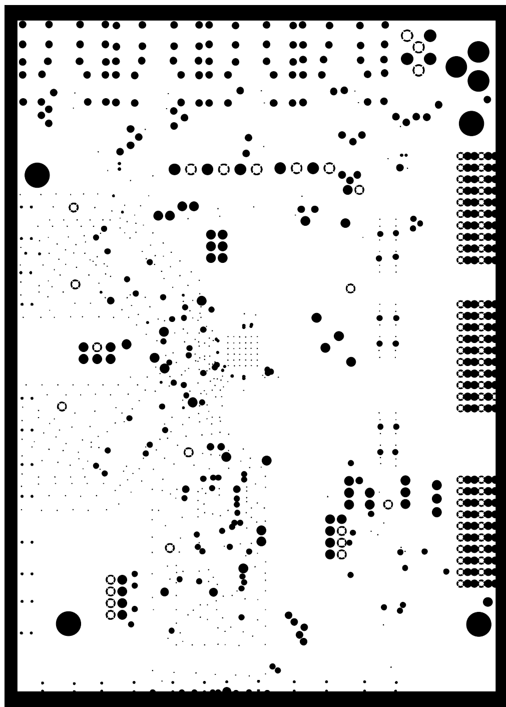
Figure 94. Evaluation Board Layout, Ground Plane
