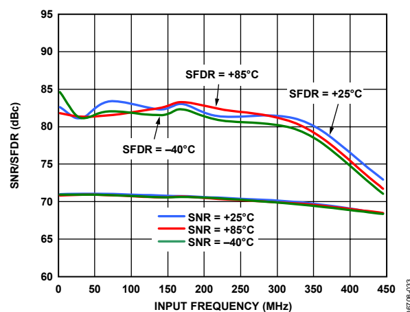
Figure 34. AD6653-125 Single-Tone SNR/SFDR vs. Input Frequency ( f_{IN} ) and Temperature with DRVDD = 3.3 V
