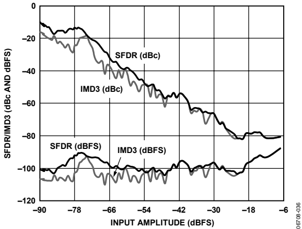
Figure 37. AD6653-150 Two-Tone SFDR/IMD3 vs. Input Amplitude ( A_{IN} ) with f_{IN1} = 169.12 MHz, f_{IN2} = 172.12 MHz, f_S = 150 MSPS, f_{NCO} = 177 MHz
