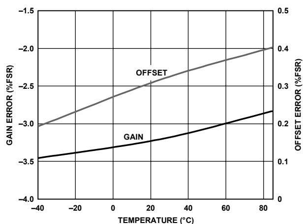
Figure 35. AD6653-150 Gain and Offset vs. Temperature
