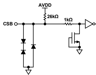
Figure 17. Equivalent CSB Input Circuit
