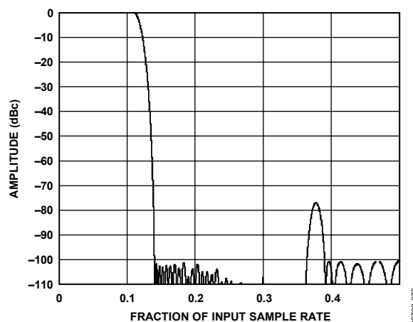
Figure 72. Half-Band Filter and FIR Filter Composite Response
