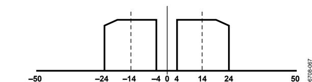
Figure 66. Example AD6653 Real 20 MHz Bandwidth Input Signal Centered at 14 MHz ( f_{\text{ADC}} = 100 MHz)
