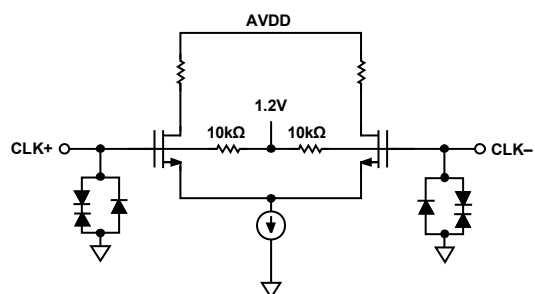
Figure 12. Equivalent Clock Input Circuit
