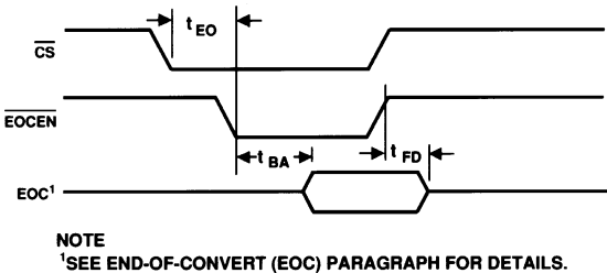
Figure 2. EOC Timing
