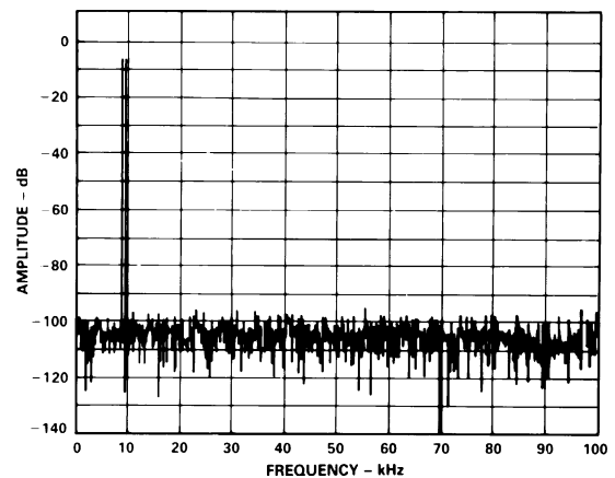
Figure 8. IMD Plot for f_{\text{IN}} = 9.08 kHz ( f_a ), 9.58 kHz ( f_b )
