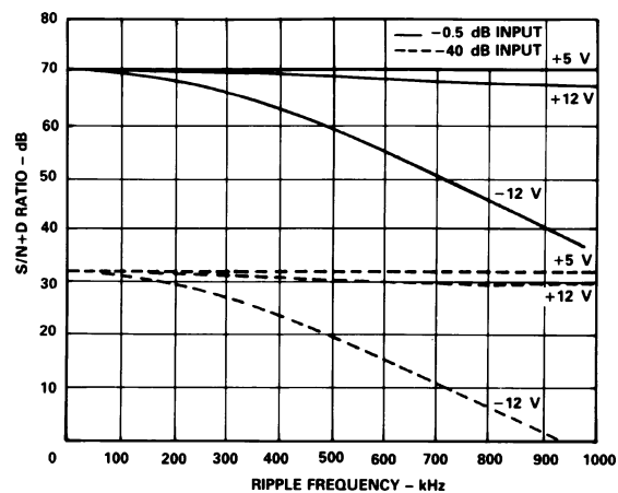
Figure 9. Power Supply Rejection ( f_{\text{IN}} = 10 kHz, f_{\text{SAMPLE}} = 200 kSPS, V_{\text{RIPPLE}} = 0.1 V p-p)
