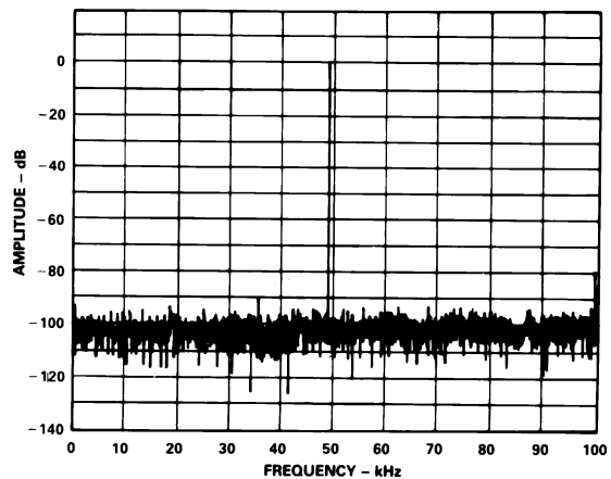
Figure 7. Nonaveraged 2048 Point FFT at 200 kSPS, f_{\text{IN}} = 49.902 kHz
