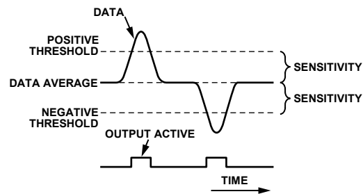
Figure 35. Threshold Sensitivity
