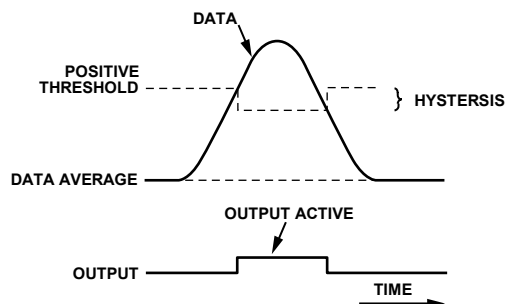
Figure 30. Threshold Hysteresis
