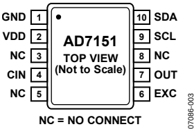
Figure 3. Pin Configuration
