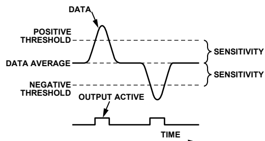
Figure 29. Threshold Sensitivity
