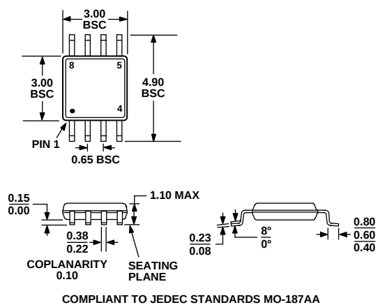
Figure 49. 8-Lead Mini Small Outline Package [MSOP] (RM-8) Dimensions shown in millimeters
