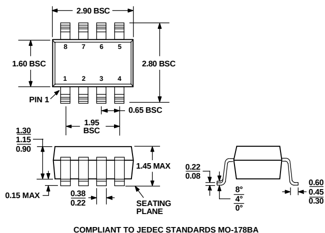
Figure 48. 8-Lead Small Outline Transistor Package [SOT-23] (RT-8) Dimensions shown in millimeters
