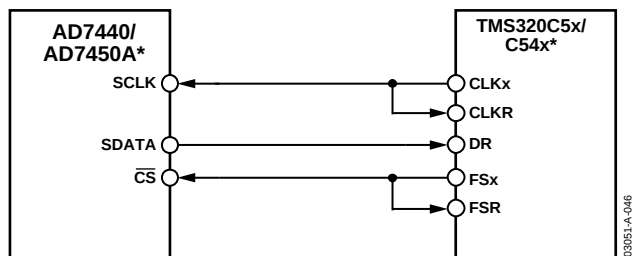
Figure 46. Interfacing to the TMS320C5x/C54x
