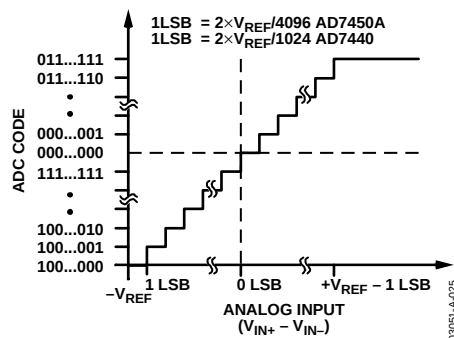
Figure 25. AD7440/AD7450A Ideal Transfer Characteristic
