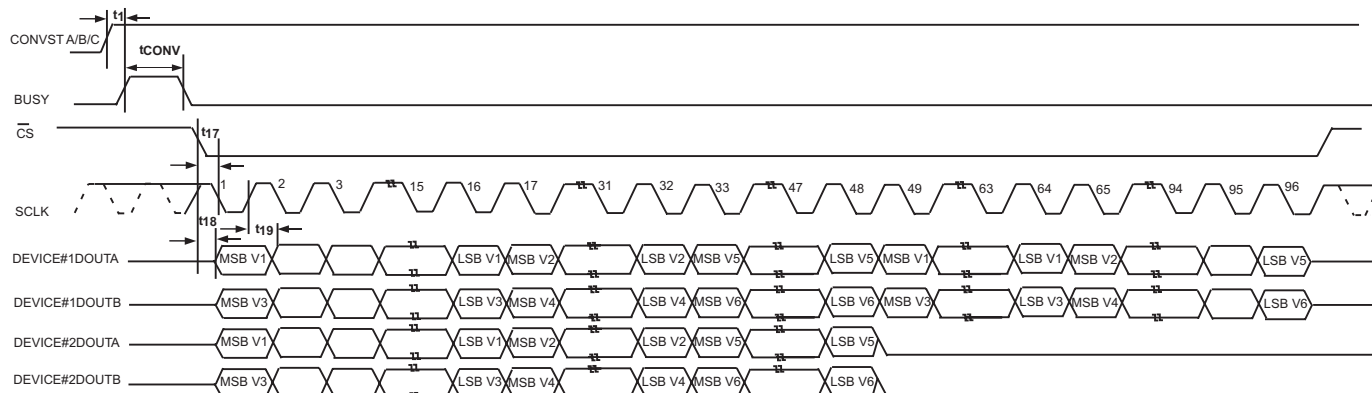
Figure 12. Daisy-Chain Configuration
