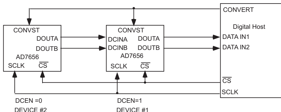
Figure 12. Daisy-Chain Configuration
