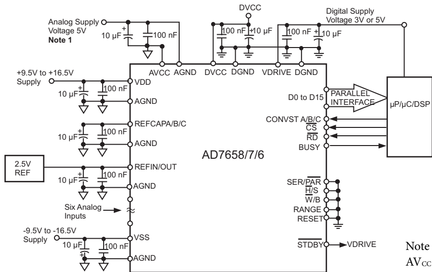
Figure 5. AD7658/AD7657/AD7656 Typical connection diagram.
