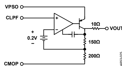
Figure 27. Output Interface
