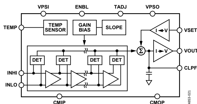
Figure 22. Block Diagram
