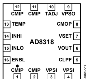
Figure 3. Pin Configuration
