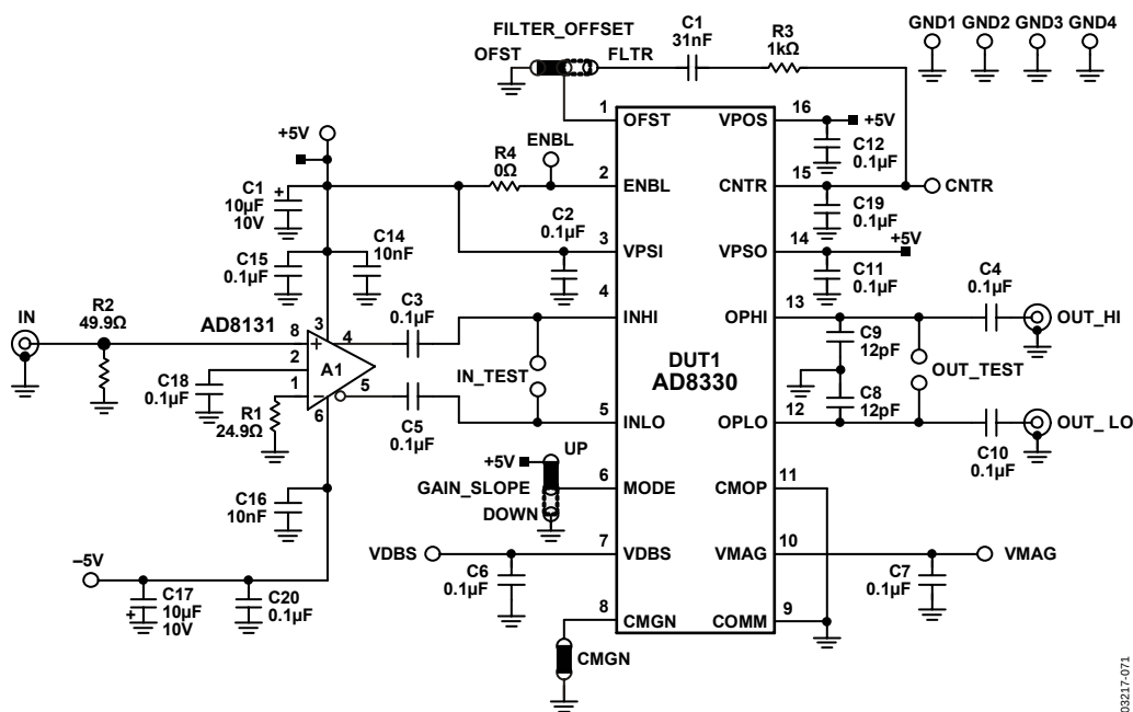
Figure 70. Schematic Diagram
