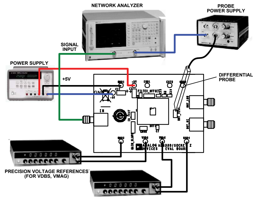
Figure 71. Typical Connections
