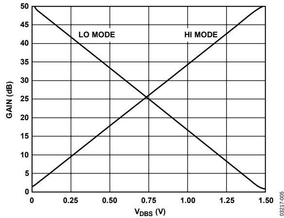
Figure 4. Gain vs. V_{DBS}
