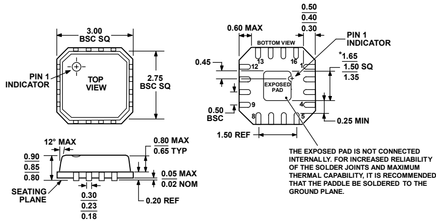
Figure 78. 16-Lead Lead Frame Chip Scale Package [LFCSP_VQ] 3 mm × 3 mm Body, Very Thin Quad (CP-16-3) Dimensions shown in millimeters
