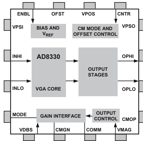
Figure 46. Block Schematic
