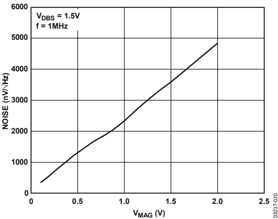
Figure 19. Output Referred Noise vs. V_{MAG}
