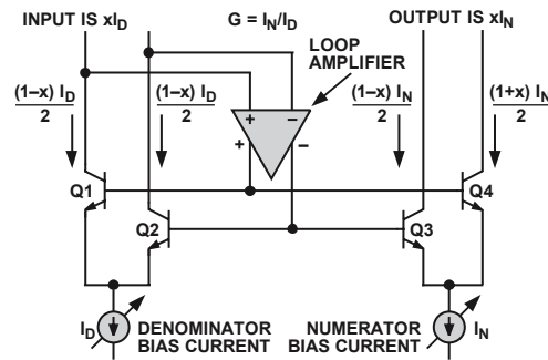
Figure 45. Basic Core
