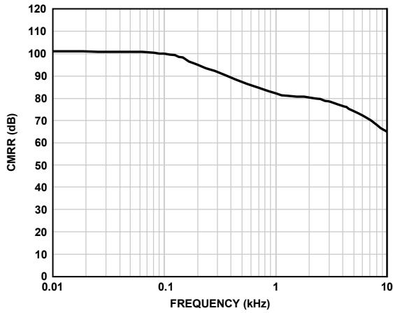
Figure 15. CMRR vs. Frequency, V_S = 5\text{ V}
