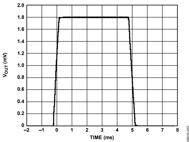
Figure 38. Large Signal Transient Response (No Load), V_S = 1.8 V
