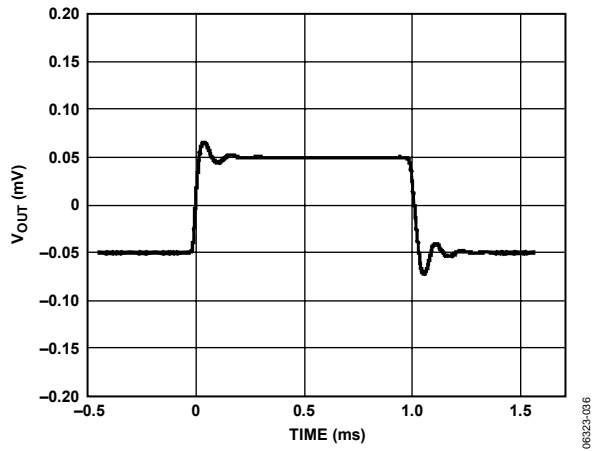
Figure 37. Small Signal Transient Response (100 pF Load Capacitance), V_S = 1.8 V
