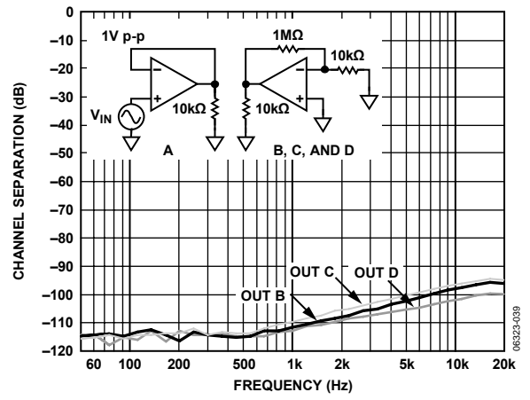
Figure 39. Channel Separation
