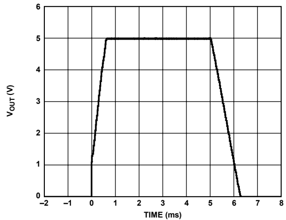
Figure 20. Large Signal Transient Response No Load, V_S = 5\text{ V}
