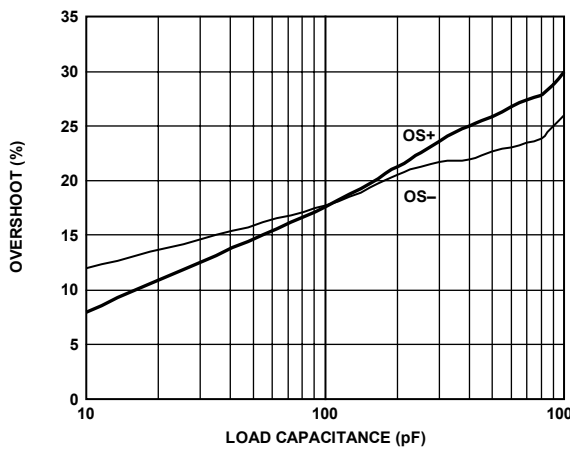
Figure 17. Small Signal Overshoot vs. Load Capacitance, V_S = 5\text{ V}
