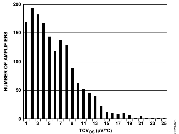
Figure 26. Input Offset Voltage Temperature Drift Distribution ( -40\text{°C} < T_A < +85\text{°C} ), V_S = 1.8\text{ V}
