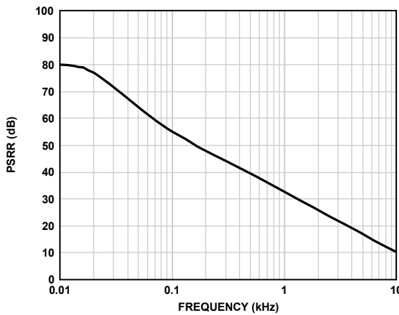
Figure 16. PSRR vs. Frequency, V_S = 5\text{ V}
