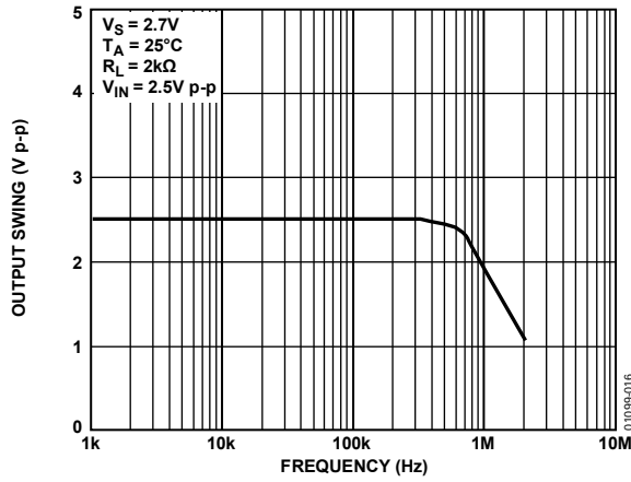
Figure 16. Closed-Loop Output Swing vs. Frequency
