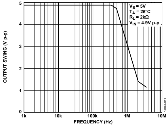
Figure 17. Closed-Loop Output Swing vs. Frequency
