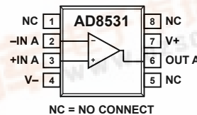
Figure 2. 8-Lead SOIC (R Suffix)
