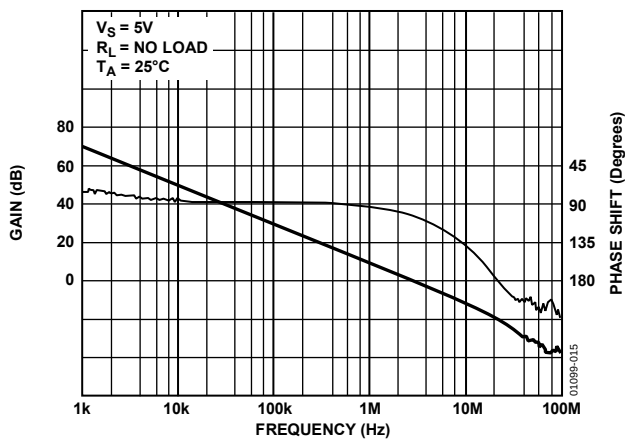
Figure 15. Open-Loop Gain and Phase Shift vs. Frequency
