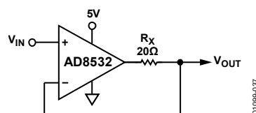
Figure 37. Output Short-Circuit Protection
