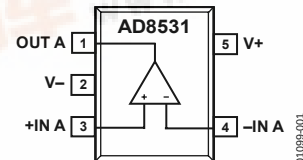
Figure 1. 5-Lead SC70 and 5-Lead SOT-23 (KS and RJ Suffixes)
