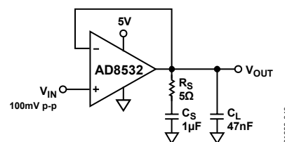
Figure 40. Snubber Network Compensates for Capacitive Loads
