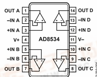
Figure 4. 14-Lead SOIC and 14-Lead TSSOP (R and RU Suffixes)
