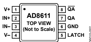
Figure 5. 8-Lead MSOP Pin Configuration
