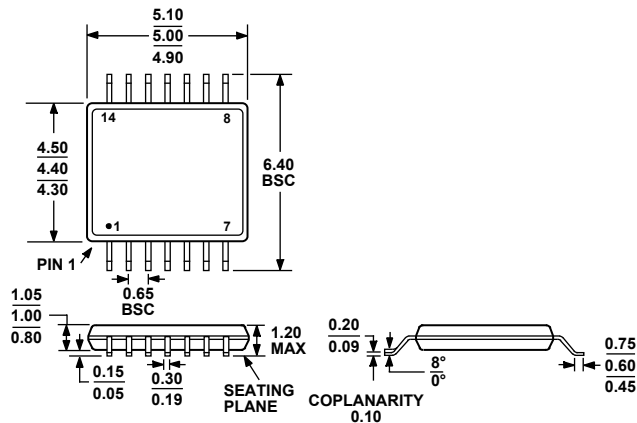
Figure 29. 14-Lead Thin Shrink Small Outline Package [TSSOP] (RU-14) Dimensions shown in millimeters
