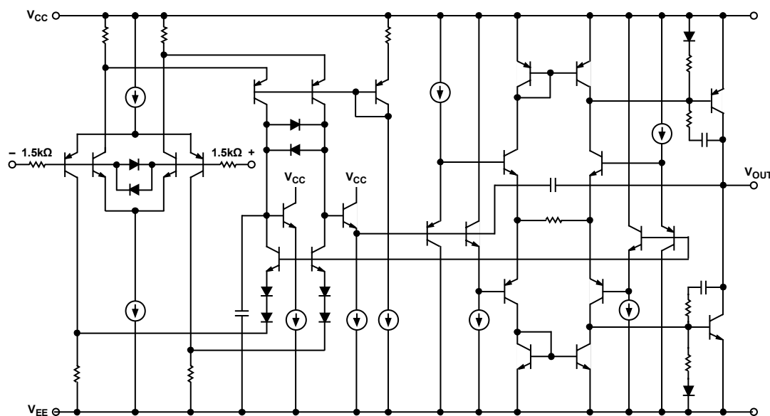
Figure 26. Simplified Schematic
