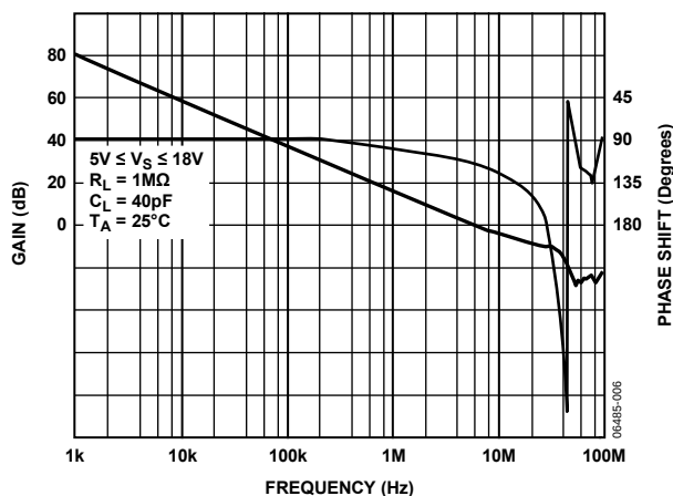
Figure 6. Open-Loop Gain and Phase Shift vs. Frequency
