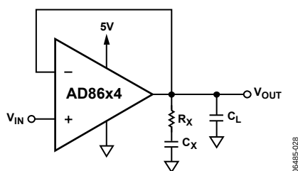
Figure 28. Snubber Network Compensation for Capacitive Loads
