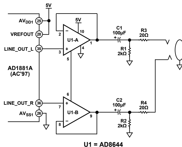
Figure 30. A PC-99-Compliant Headphone/Line Out Amplifier
