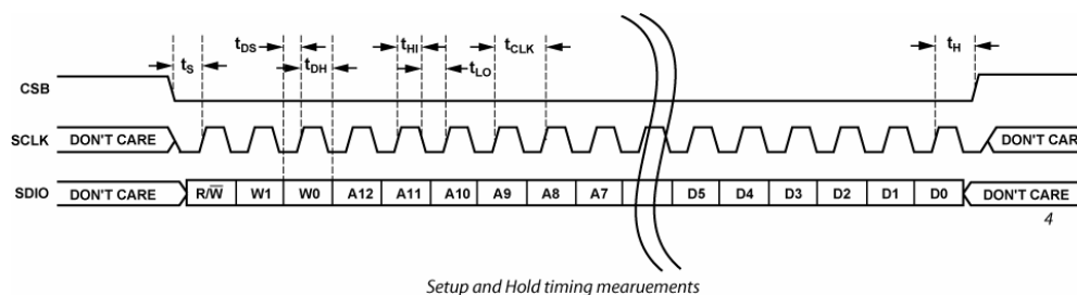
Figure X. Serial Port Interface Timing Diagram
