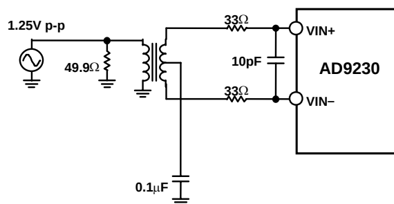
Figure 15. Differential Transformer—Coupled Configuration
