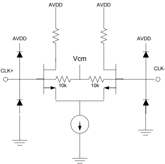
Figure 4 Clock Inputs
