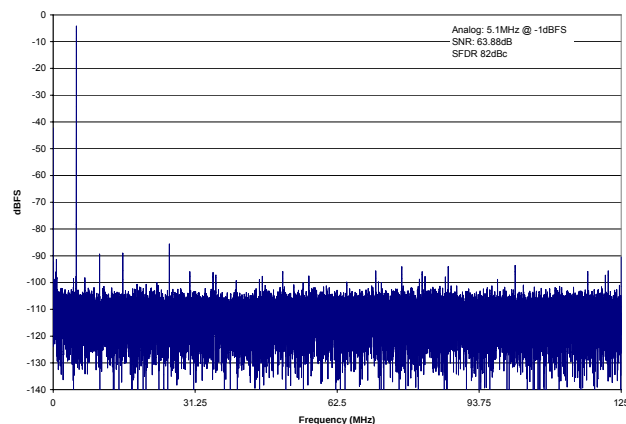
Figure 11. AD9230-250 64k Point Single-Tone FFT/250 MSPS 5.1 MHz
