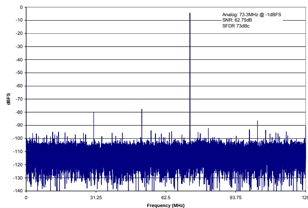
Figure 13. AD9230-250 64k Point Single-Tone FFT/250 MSPS 70.3 MHz
