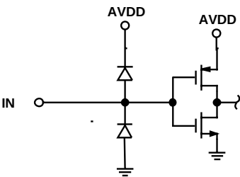
Figure 6. Logic Inputs
