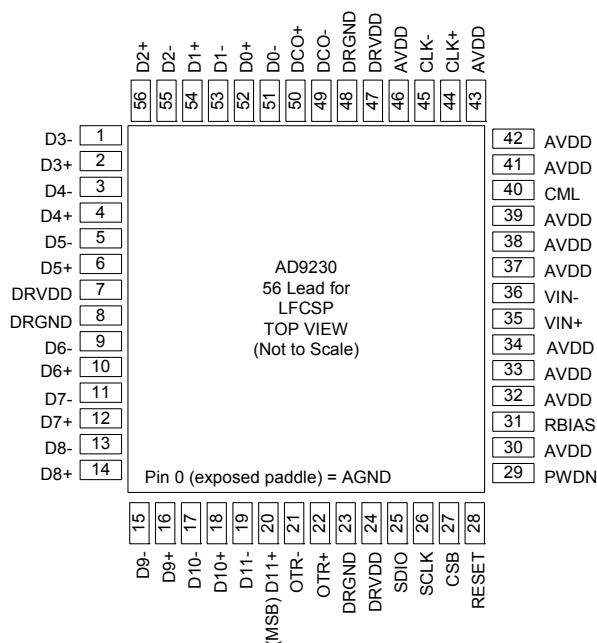
Figure 3. Pinout )
