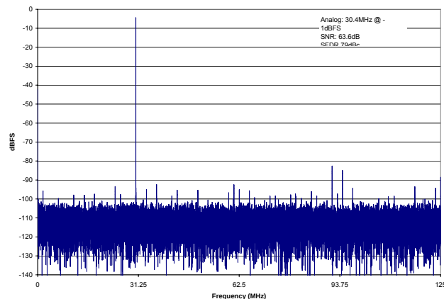
Figure 12. AD9230-250 64k Point Single-Tone FFT/250 MSPS 30.3 MHz
