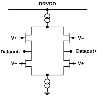
Figure 7. Data Outputs (LVDS Mode)
