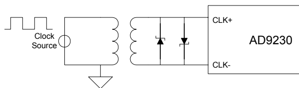
Figure X. Transformer Coupled Differential Clock
