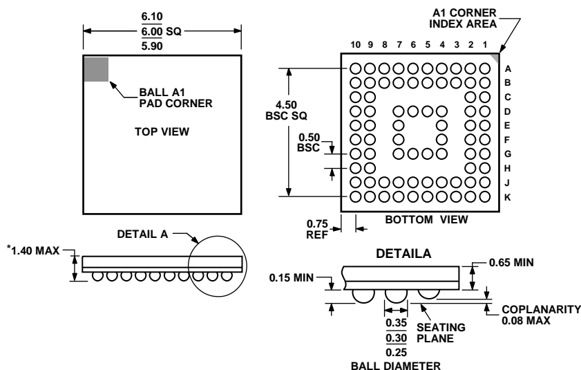
Figure 8. 76-Ball Chip Scale Package Ball Grid Array [CSP_BGA] 6 mm × 6 mm × 1.4 mm (BC-76)
