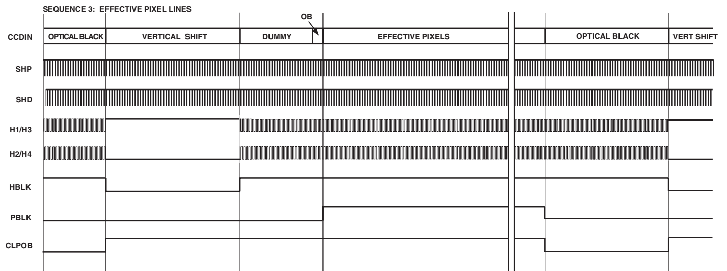
Figure 27. Horizontal Sequences during Effective Pixels
