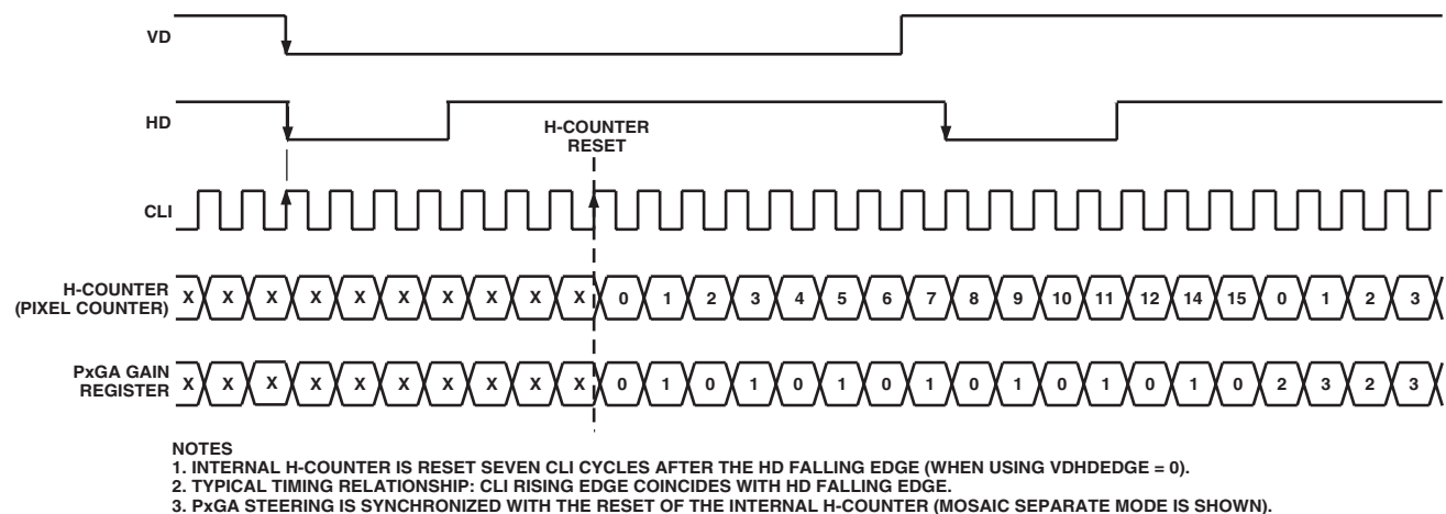
Figure 13. H-Counter Synchronization
