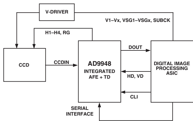
Figure 1. Typical Application
