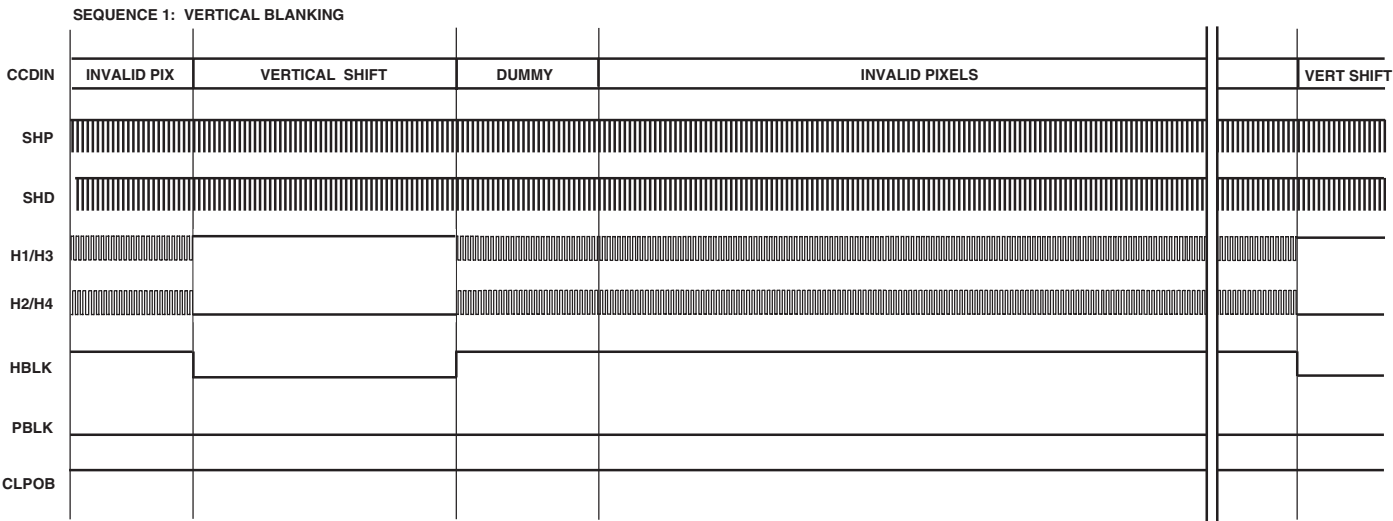
Figure 25. Horizontal Sequence during Vertical Blanking
