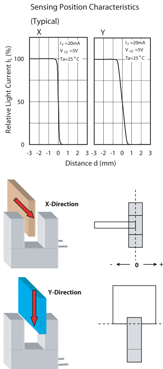
Figure 2: Illustrates Photo-Interrupter Positioning Sensing Characteristics. Obstacles (Slots) could interrupt along X-axis or Y-axis
