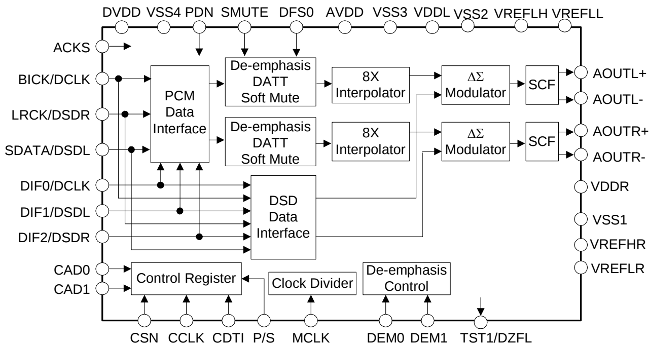
Block Diagram
