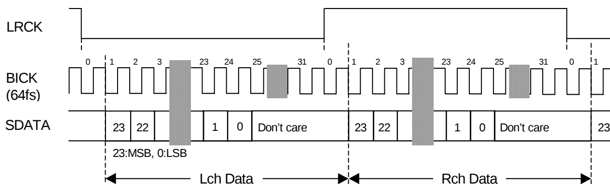
Figure 4. Mode 3 Timing
