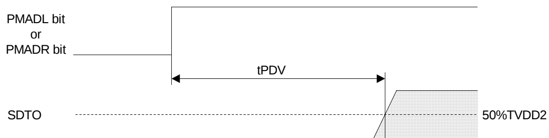
Figure 16. Power Down &amp; Reset Timing 1
