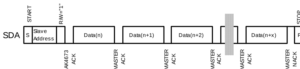
Figure 81. CURRENT ADDRESS READ
