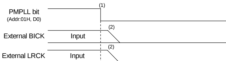
Figure 94. Clock Stopping Sequence (2)
