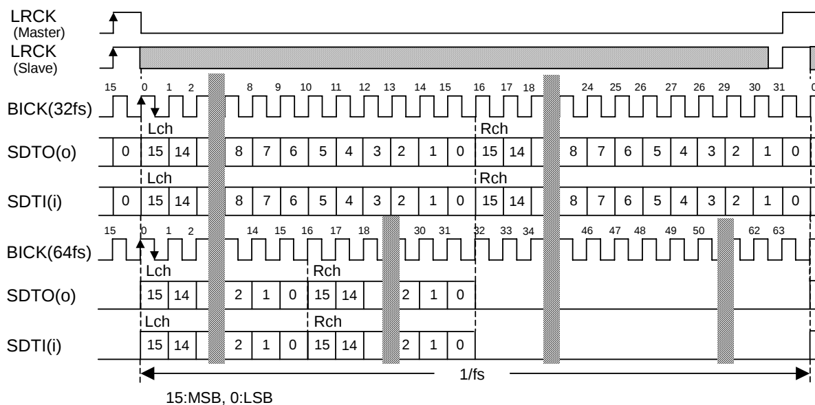
Figure 26. Mode 0 Timing (BCKP = "0", MSBS = "1")
