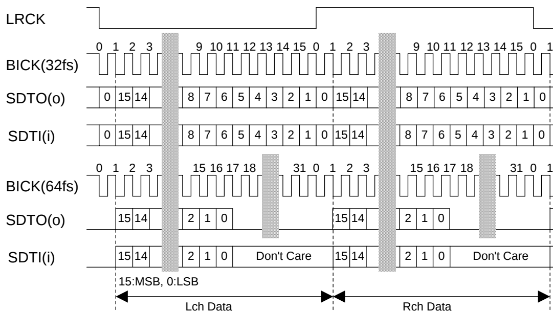
Figure 30. Mode 3 Timing
