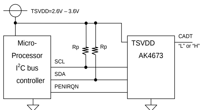
Figure 65 Digital I/F
