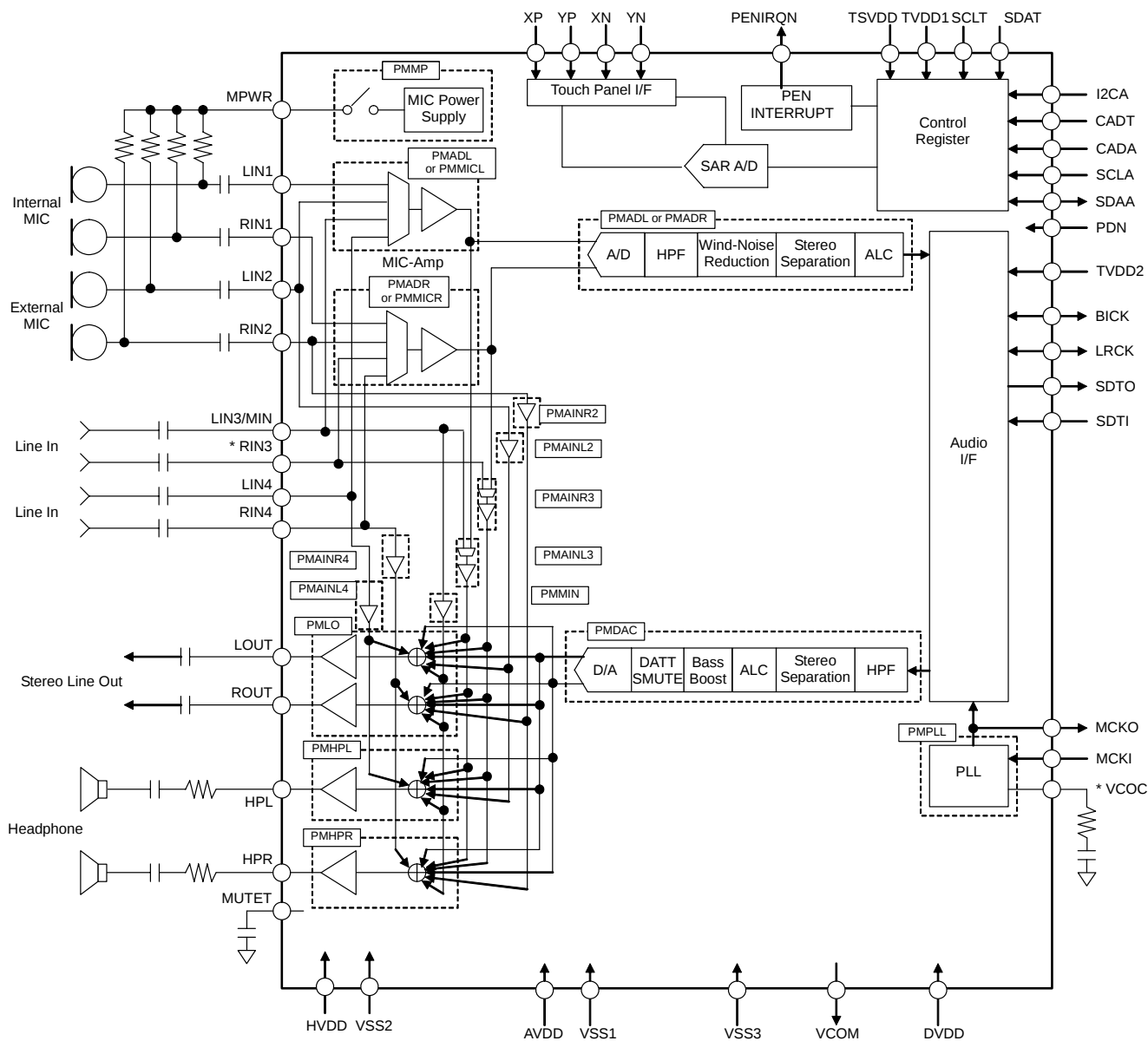
(VCOC and RIN3 pins are shared by the same pin.) Figure 1. Block Diagram
