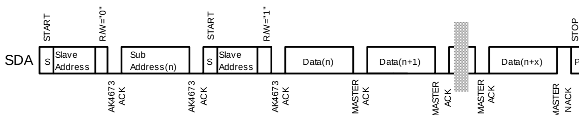
Figure 82. RANDOM ADDRESS READ
