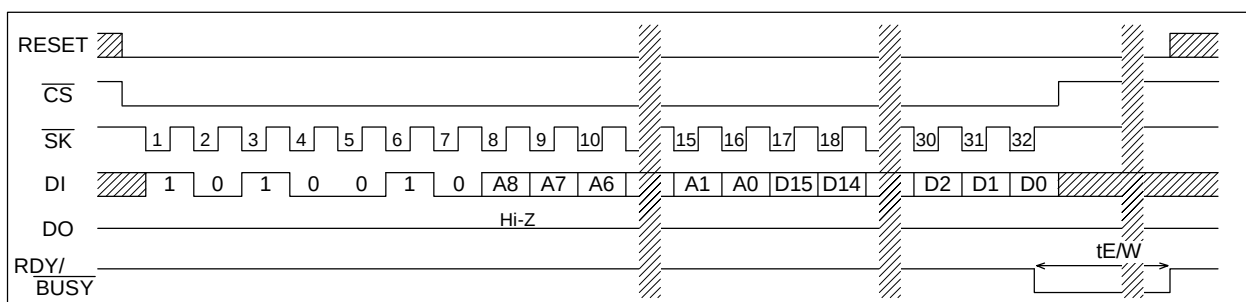
WRITE (AK6480C)
