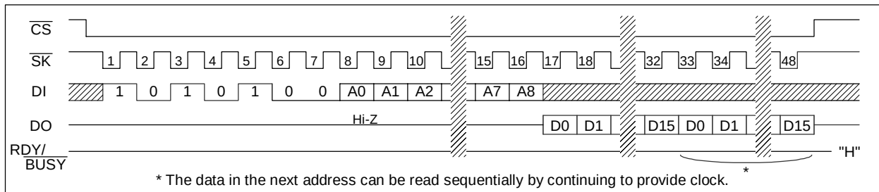
READ (AK6481C)
