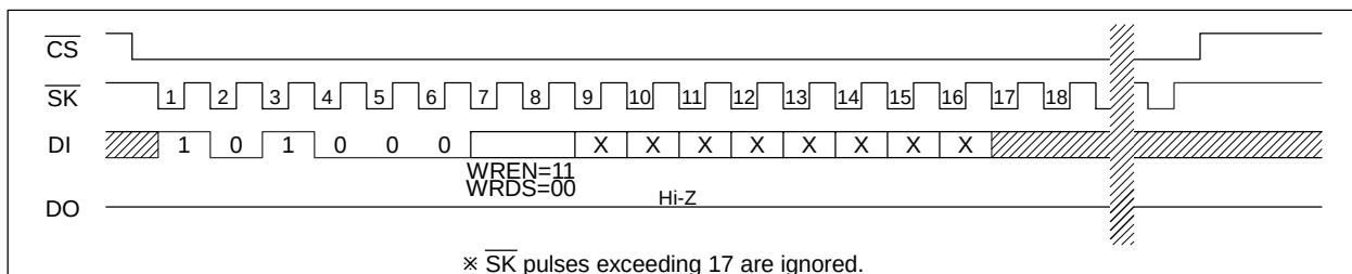
WREN / WRDS
