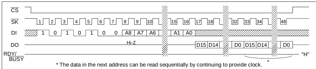
READ (AK6480C)
