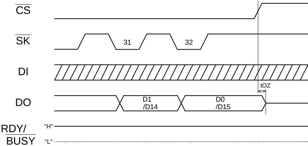
Upper:AK6480C, Lower:AK6481C Data Output (READ)
