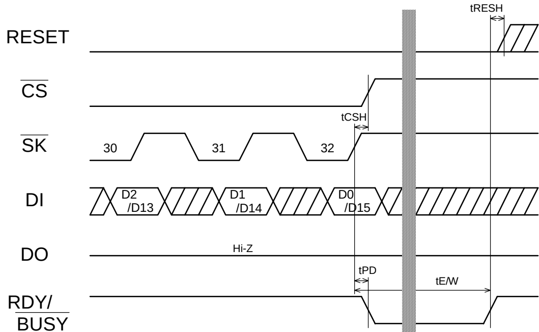
Upper:AK6480C, Lower:AK6481C WRITE Ready / \overline{Busy} Signal Output ( \overline{RDY}/\overline{BUSY} pin)
