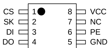
8pin TMSOP
