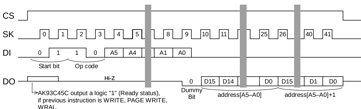
READ (AK93C45C)
