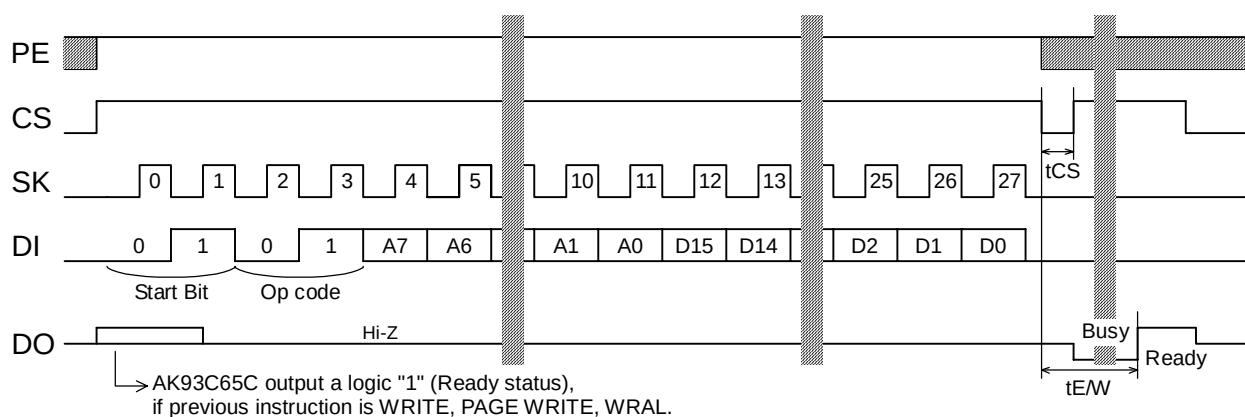
WRITE (AK93C65C)
