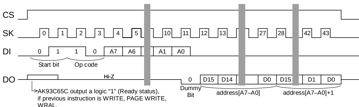
READ (AK93C65C)
