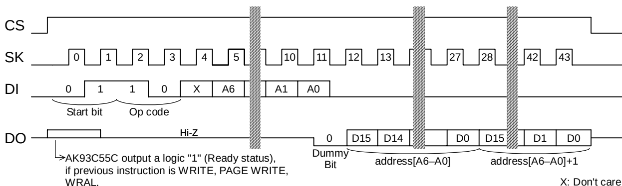
READ (AK93C55C)
