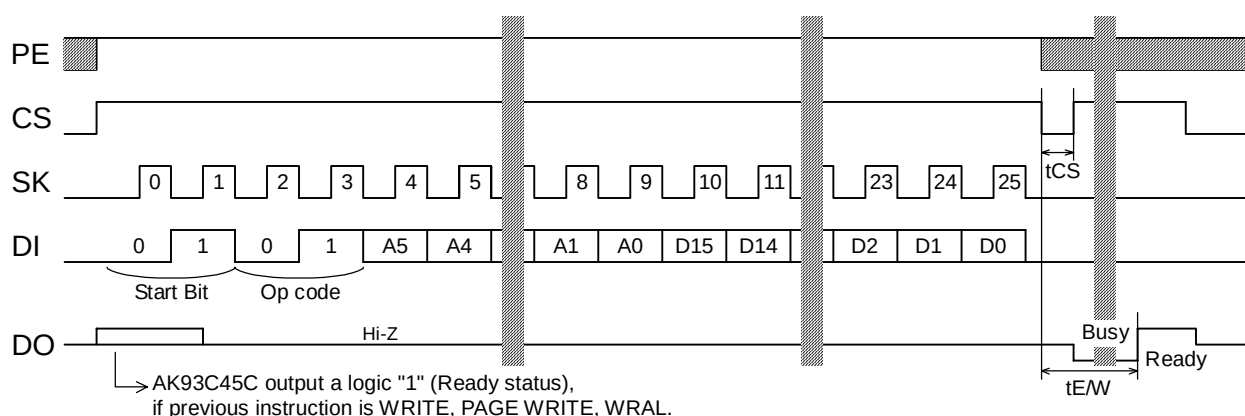
WRITE (AK93C45C)
