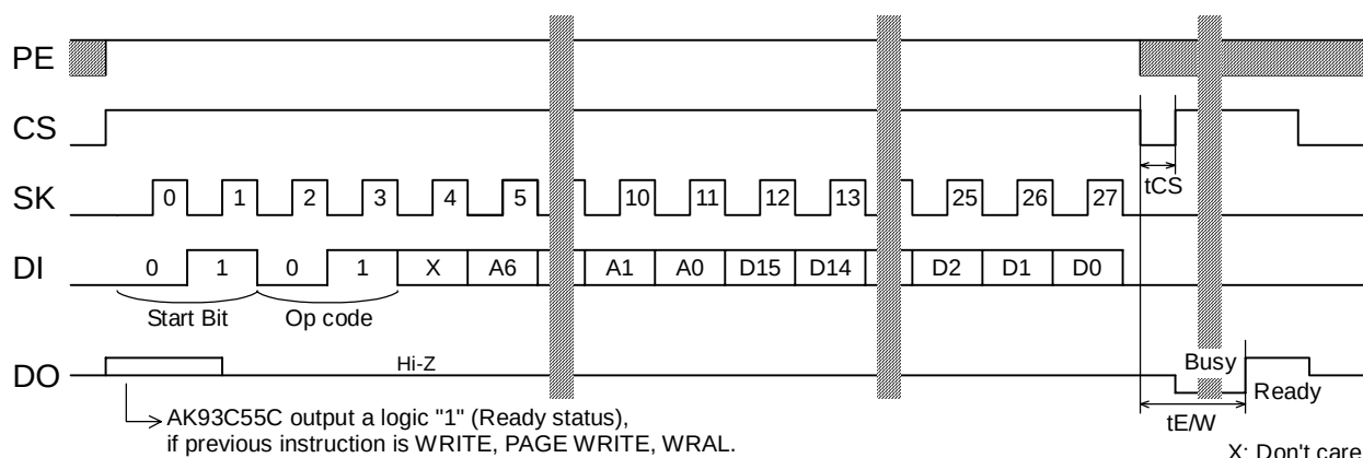
WRITE (AK93C55C)
