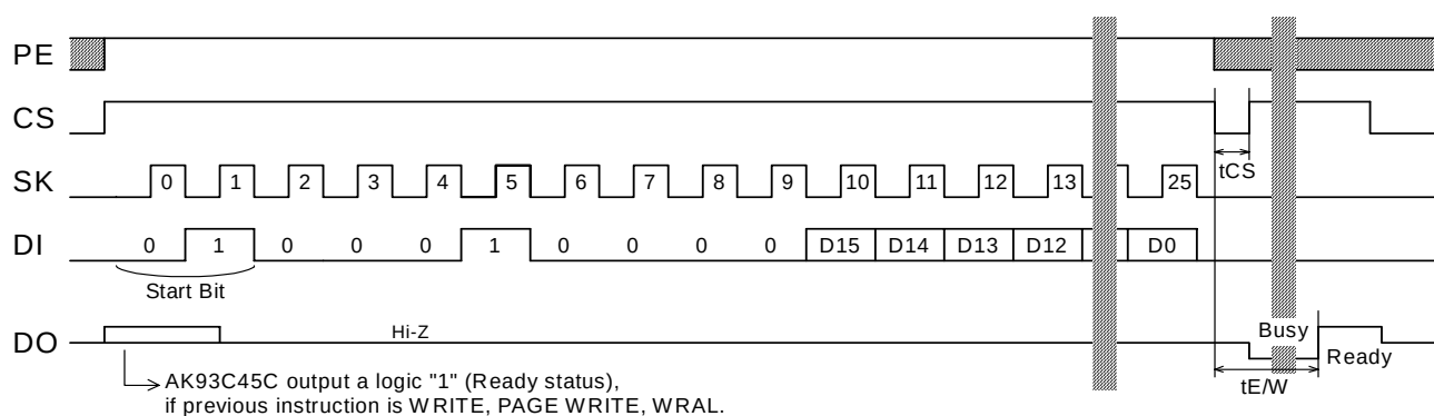
WRAL (AK93C45C)
