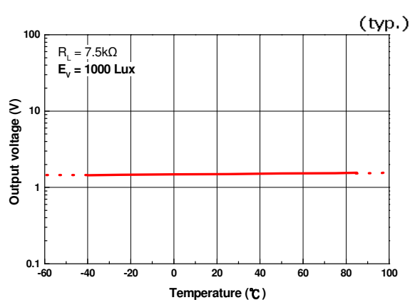
Fig.10 Output voltage vs. Temperature
