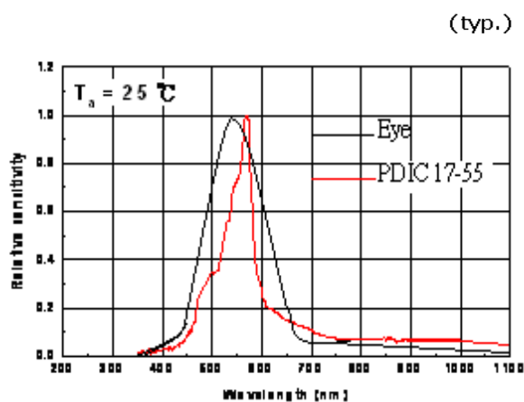
Fig.9 Spectral Response
